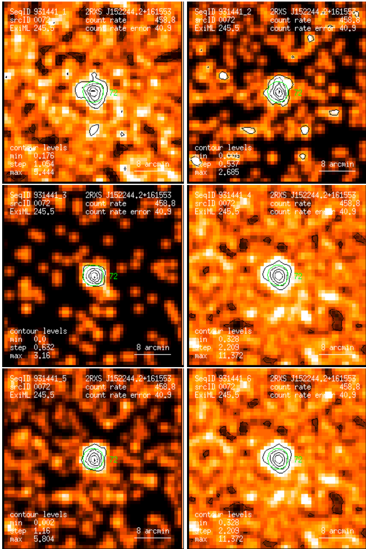
Figure 72: RASS 931441: detection 0072: band rate images, Gaussian filter: (1) PSPC channels 11 – 41, (2) 52 – 90, (3) 91 – 201, (4) 11 – 235, (5) 52 – 201, (6) 11 – 201. Broad band rates in counts/ks. Band rate contour levels in counts/ks/arcmin 2 .
