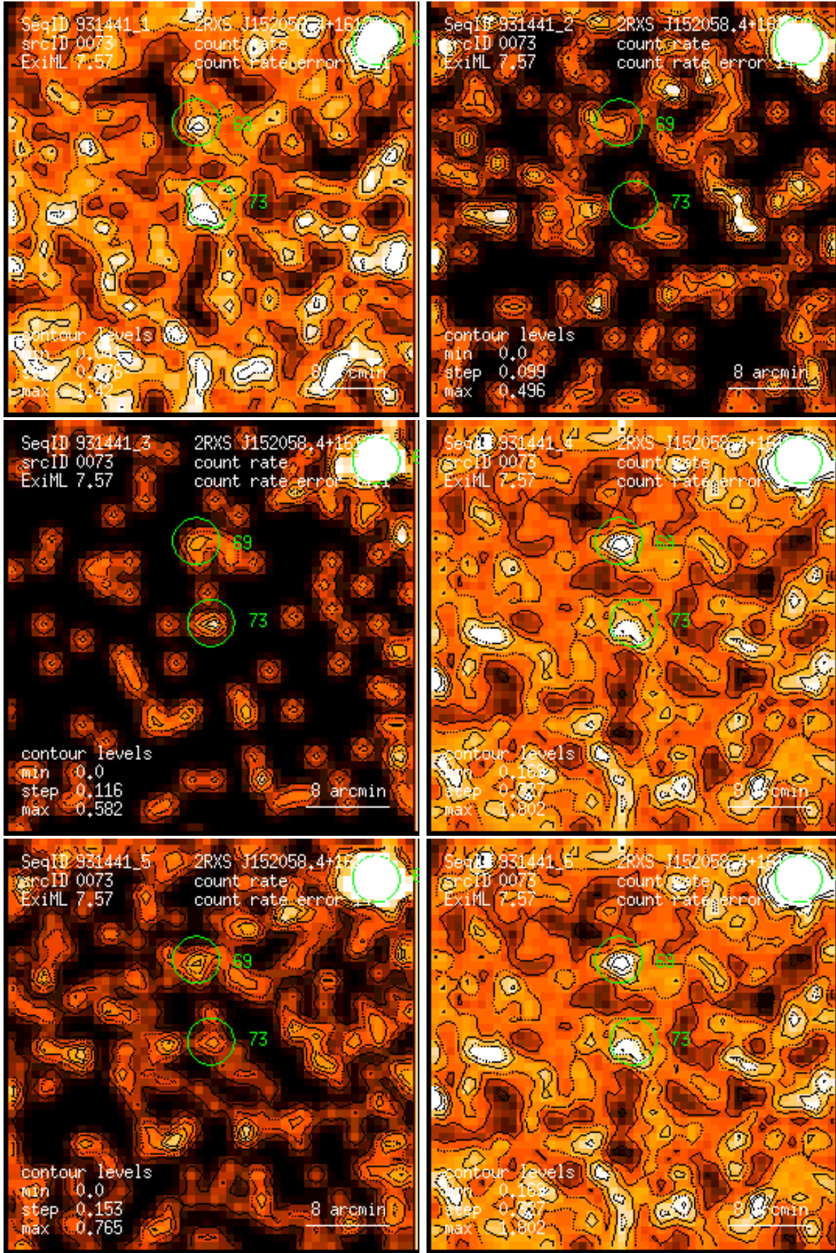
Figure 73: RASS 931441: detection 0073: band rate images, Gaussian filter: (1) PSPC channels 11 – 41, (2) 52 – 90, (3) 91 – 201, (4) 11 – 235, (5) 52 – 201, (6) 11 – 201. Broad band rates in counts/ks. Band rate contour levels in counts/ks/arcmin 2 .
