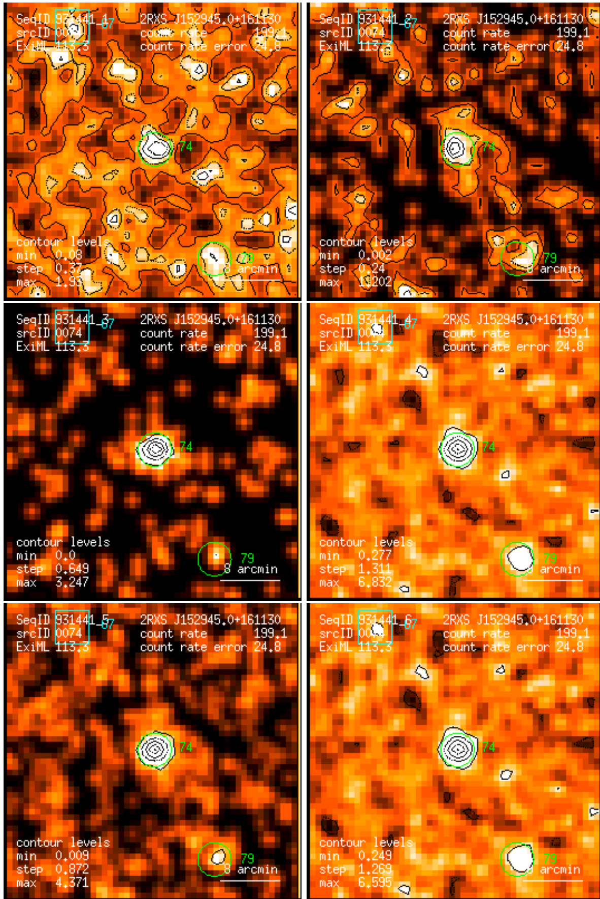
Figure 74: RASS 931441: detection 0074: band rate images, Gaussian filter: (1) PSPC channels 11 – 41, (2) 52 – 90, (3) 91 – 201, (4) 11 – 235, (5) 52 – 201, (6) 11 – 201. Broad band rates in counts/ks. Band rate contour levels in counts/ks/arcmin 2 .
