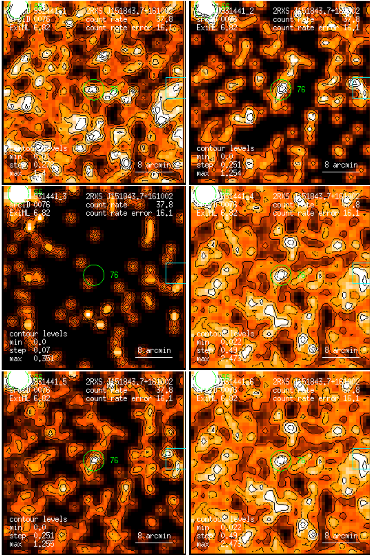
Figure 76: RASS 931441: detection 0076: band rate images, Gaussian filter: (1) PSPC channels 11 – 41, (2) 52 – 90, (3) 91 – 201, (4) 11 – 235, (5) 52 – 201, (6) 11 – 201. Broad band rates in counts/ks. Band rate contour levels in counts/ks/arcmin 2 .
