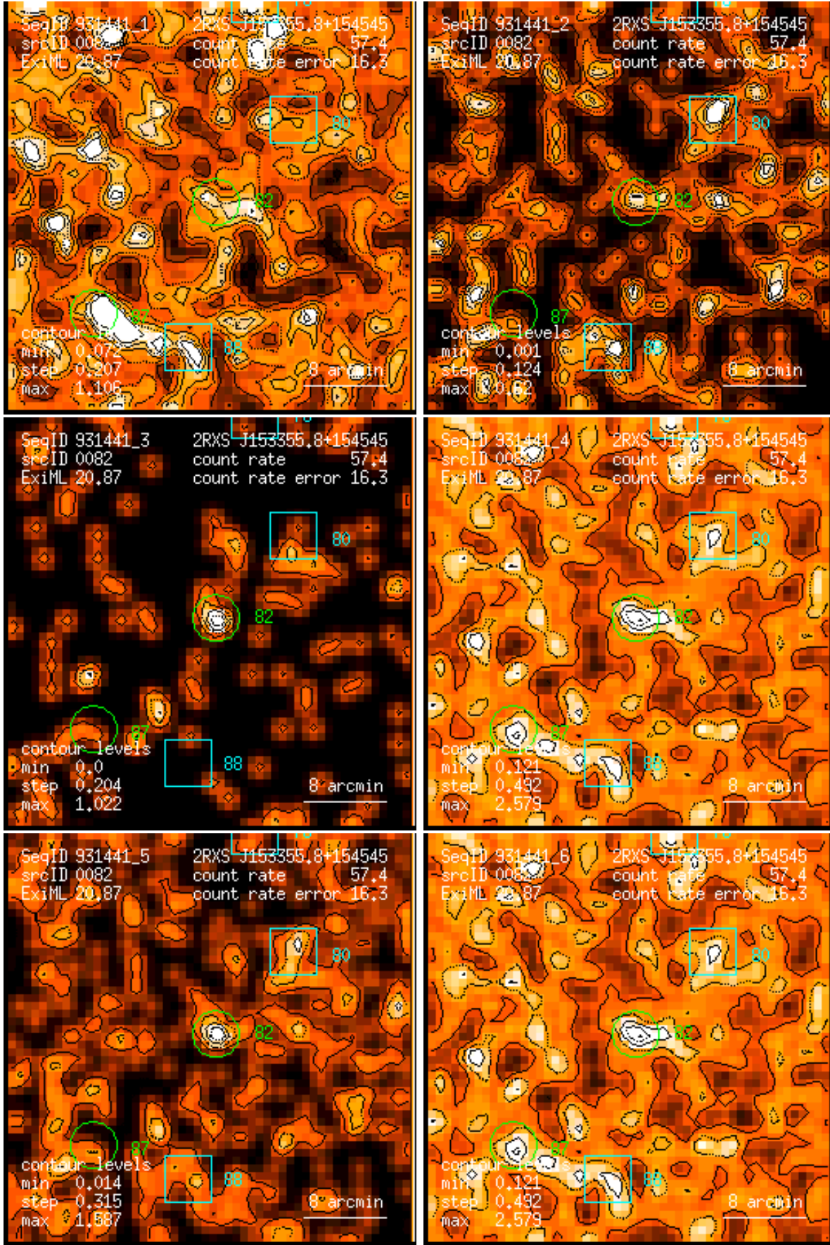
Figure 82: RASS 931441: detection 0082: band rate images, Gaussian filter: (1) PSPC channels 11 – 41, (2) 52 – 90, (3) 91 – 201, (4) 11 – 235, (5) 52 – 201, (6) 11 – 201. Broad band rates in counts/ks. Band rate contour levels in counts/ks/arcmin 2 .
