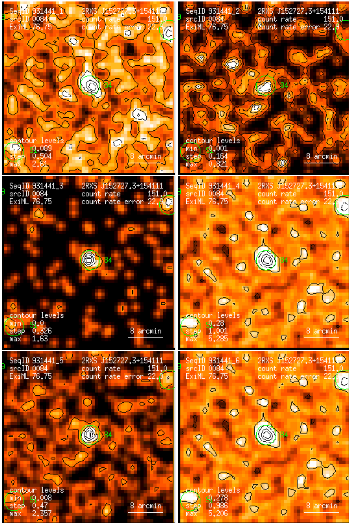
Figure 84: RASS 931441: detection 0084: band rate images, Gaussian filter: (1) PSPC channels 11 – 41, (2) 52 – 90, (3) 91 – 201, (4) 11 – 235, (5) 52 – 201, (6) 11 – 201. Broad band rates in counts/ks. Band rate contour levels in counts/ks/arcmin 2 .
