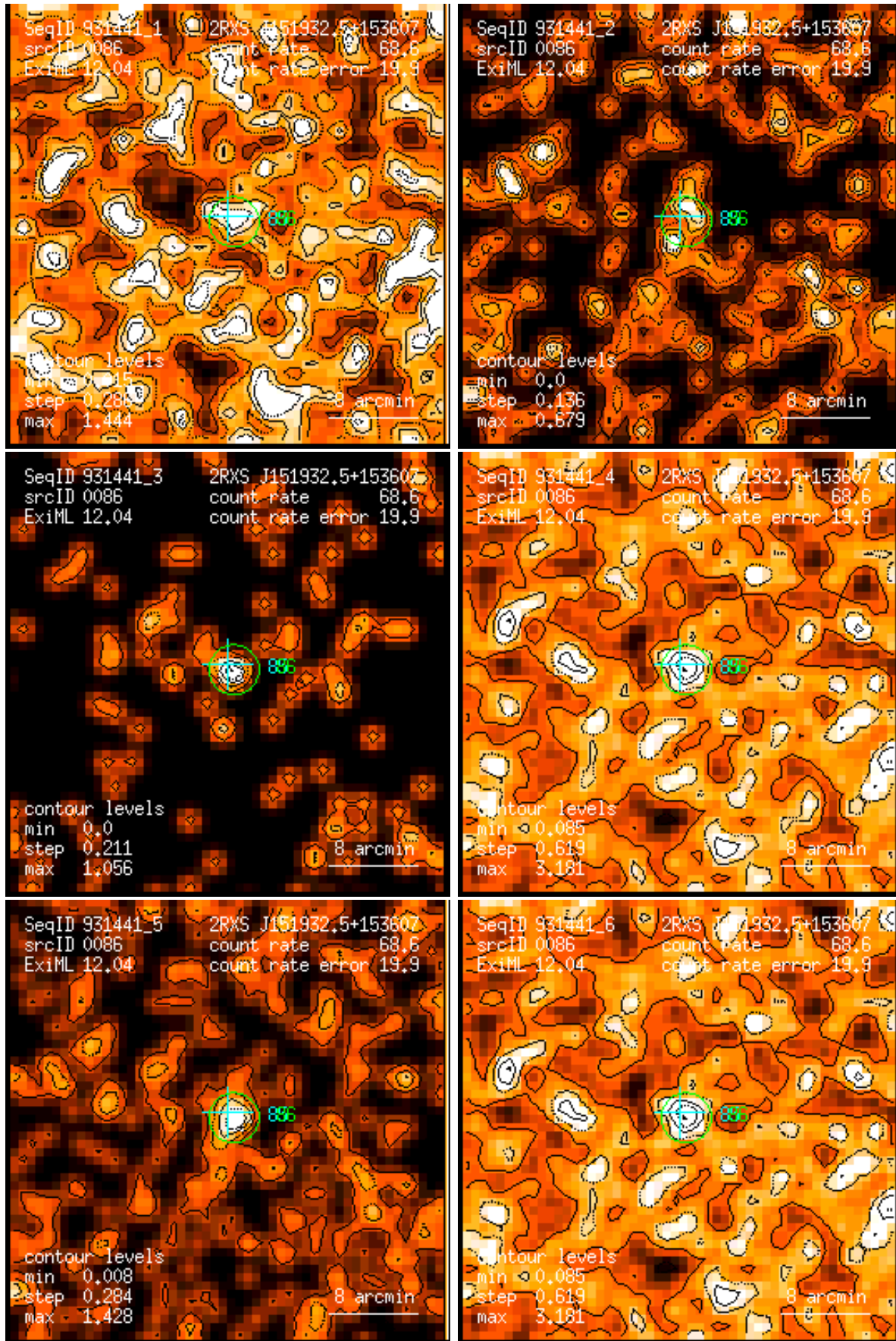
Figure 86: RASS 931441: detection 0086: band rate images, Gaussian filter: (1) PSPC channels 11 – 41, (2) 52 – 90, (3) 91 – 201, (4) 11 – 235, (5) 52 – 201, (6) 11 – 201. Broad band rates in counts/ks. Band rate contour levels in counts/ks/arcmin 2 .
