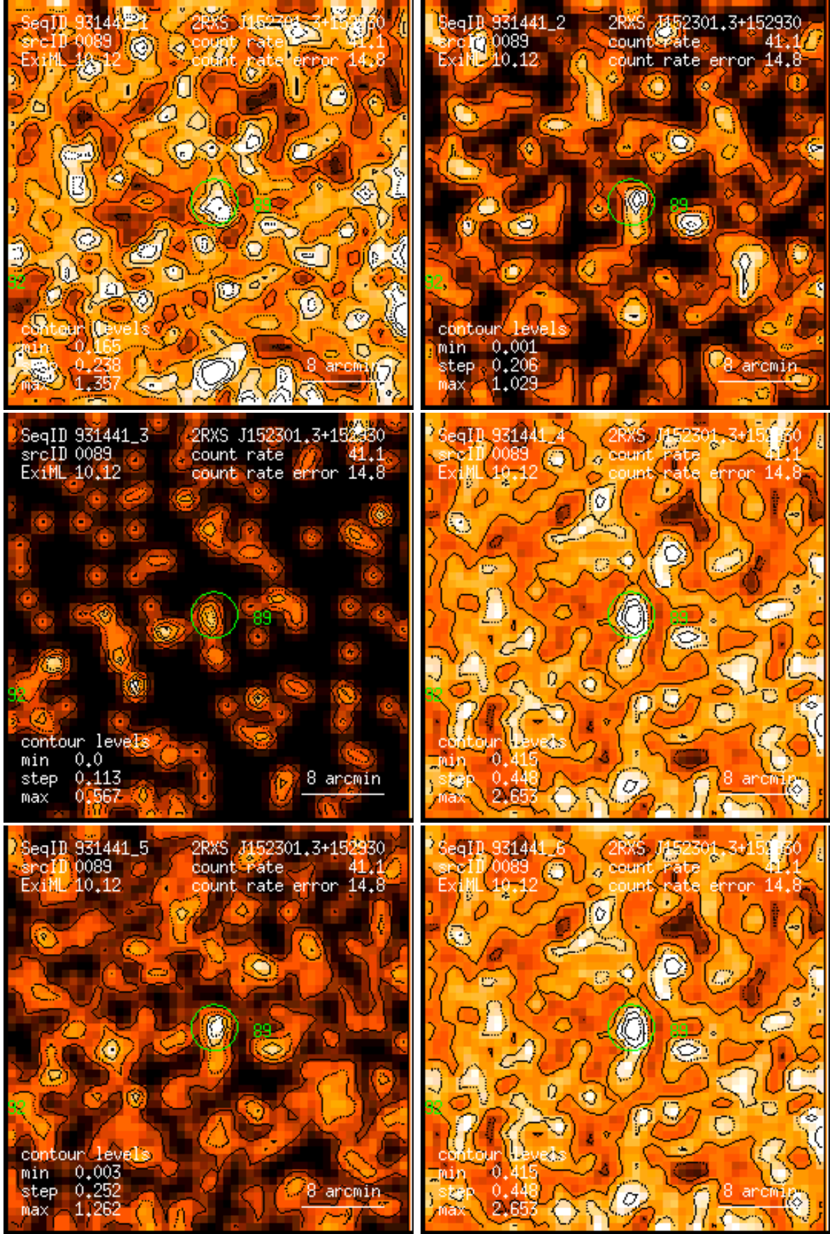
Figure 89: RASS 931441: detection 0089: band rate images, Gaussian filter: (1) PSPC channels 11 – 41, (2) 52 – 90, (3) 91 – 201, (4) 11 – 235, (5) 52 – 201, (6) 11 – 201. Broad band rates in counts/ks. Band rate contour levels in counts/ks/arcmin 2 .
