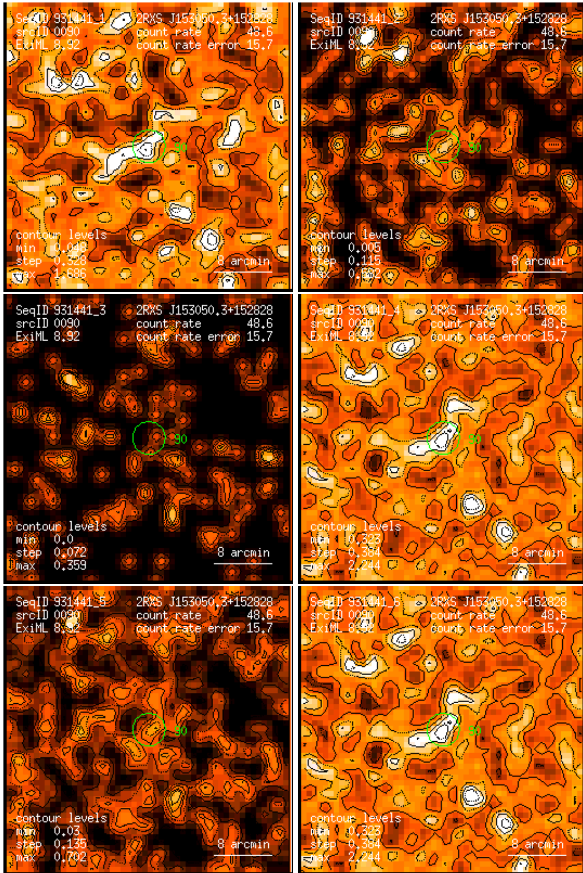
Figure 90: RASS 931441: detection 0090: band rate images, Gaussian filter: (1) PSPC channels 11 – 41, (2) 52 – 90, (3) 91 – 201, (4) 11 – 235, (5) 52 – 201, (6) 11 – 201. Broad band rates in counts/ks. Band rate contour levels in counts/ks/arcmin 2 .
