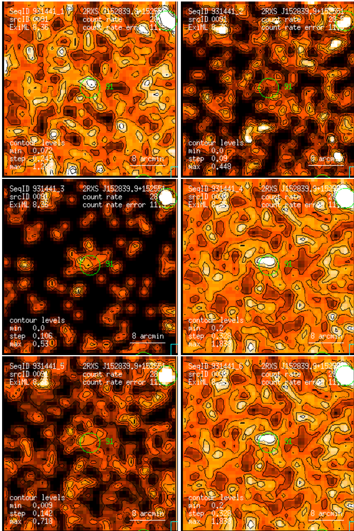
Figure 91: RASS 931441: detection 0091: band rate images, Gaussian filter: (1) PSPC channels 11 – 41, (2) 52 – 90, (3) 91 – 201, (4) 11 – 235, (5) 52 – 201, (6) 11 – 201. Broad band rates in counts/ks. Band rate contour levels in counts/ks/arcmin 2 .
