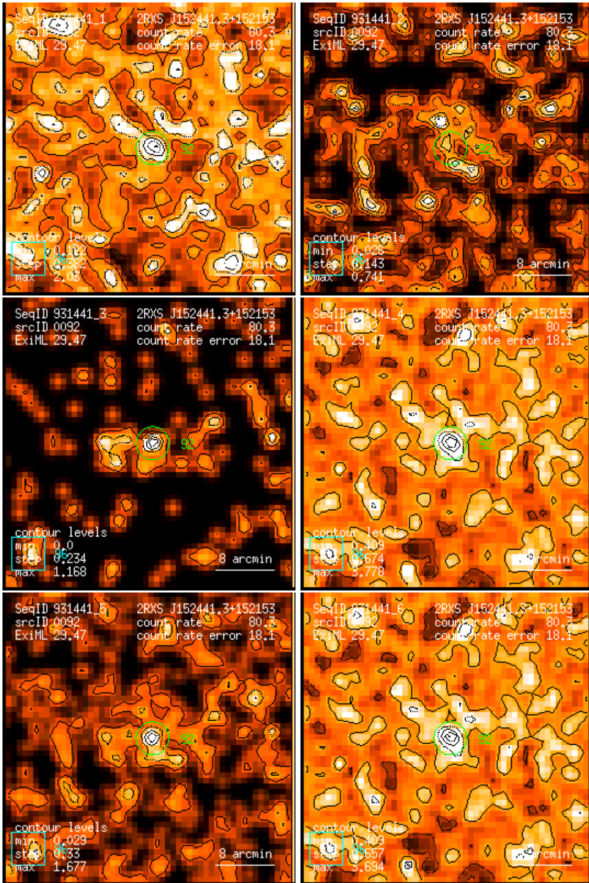
Figure 92: RASS 931441: detection 0092: band rate images, Gaussian filter: (1) PSPC channels 11 – 41, (2) 52 – 90, (3) 91 – 201, (4) 11 – 235, (5) 52 – 201, (6) 11 – 201. Broad band rates in counts/ks. Band rate contour levels in counts/ks/arcmin 2 .
