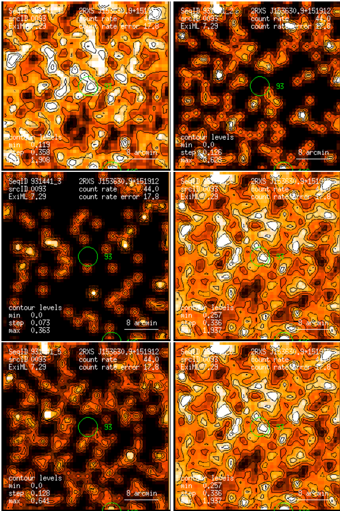
Figure 93: RASS 931441: detection 0093: band rate images, Gaussian filter: (1) PSPC channels 11 – 41, (2) 52 – 90, (3) 91 – 201, (4) 11 – 235, (5) 52 – 201, (6) 11 – 201. Broad band rates in counts/ks. Band rate contour levels in counts/ks/arcmin 2 .
