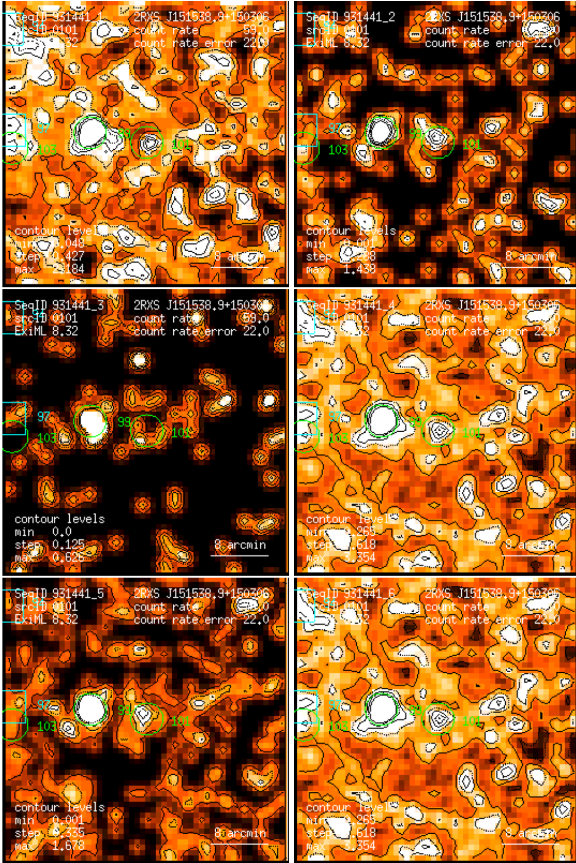
Figure 101: RASS 931441: detection 0101: band rate images, Gaussian filter: (1) PSPC channels 11 – 41, (2) 52 – 90, (3) 91 – 201, (4) 11 – 235, (5) 52 – 201, (6) 11 – 201. Broad band rates in counts/ks. Band rate contour levels in counts/ks/arcmin 2 .
