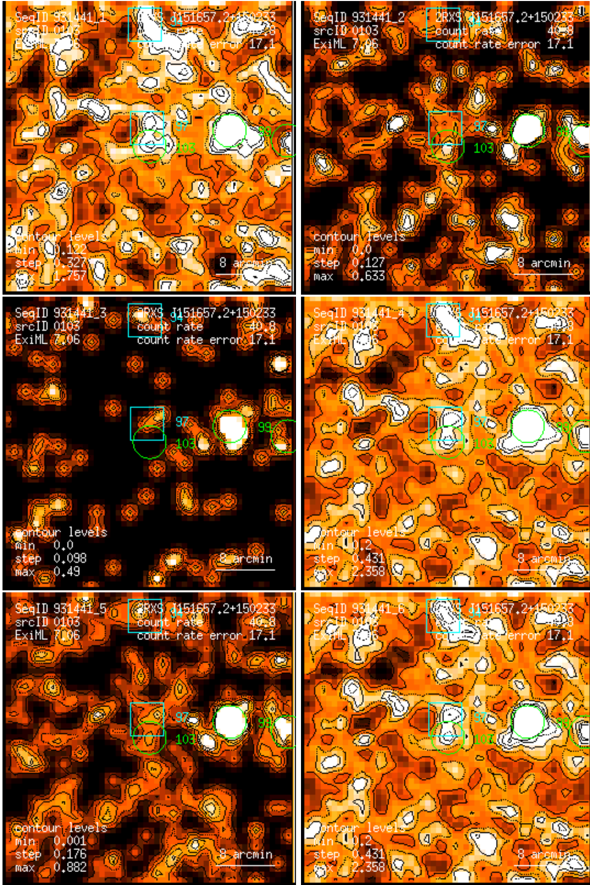
Figure 103: RASS 931441: detection 0103: band rate images, Gaussian filter: (1) PSPC channels 11 – 41, (2) 52 – 90, (3) 91 – 201, (4) 11 – 235, (5) 52 – 201, (6) 11 – 201. Broad band rates in counts/ks. Band rate contour levels in counts/ks/arcmin 2 .
