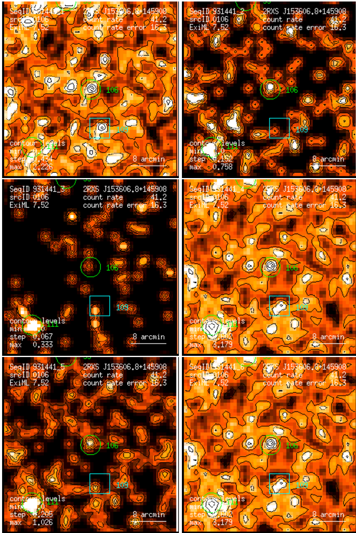
Figure 106: RASS 931441: detection 0106: band rate images, Gaussian filter: (1) PSPC channels 11 – 41, (2) 52 – 90, (3) 91 – 201, (4) 11 – 235, (5) 52 – 201, (6) 11 – 201. Broad band rates in counts/ks. Band rate contour levels in counts/ks/arcmin 2 .
