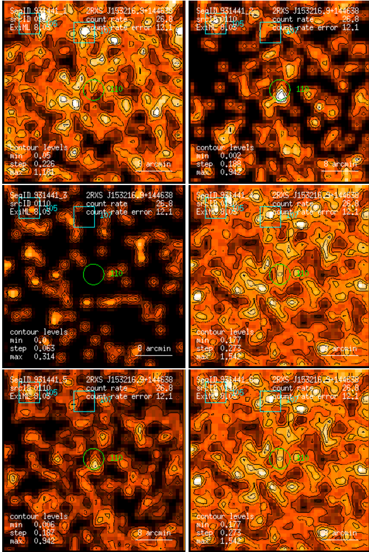
Figure 110: RASS 931441: detection 0110: band rate images, Gaussian filter: (1) PSPC channels 11 – 41, (2) 52 – 90, (3) 91 – 201, (4) 11 – 235, (5) 52 – 201, (6) 11 – 201. Broad band rates in counts/ks. Band rate contour levels in counts/ks/arcmin 2 .
