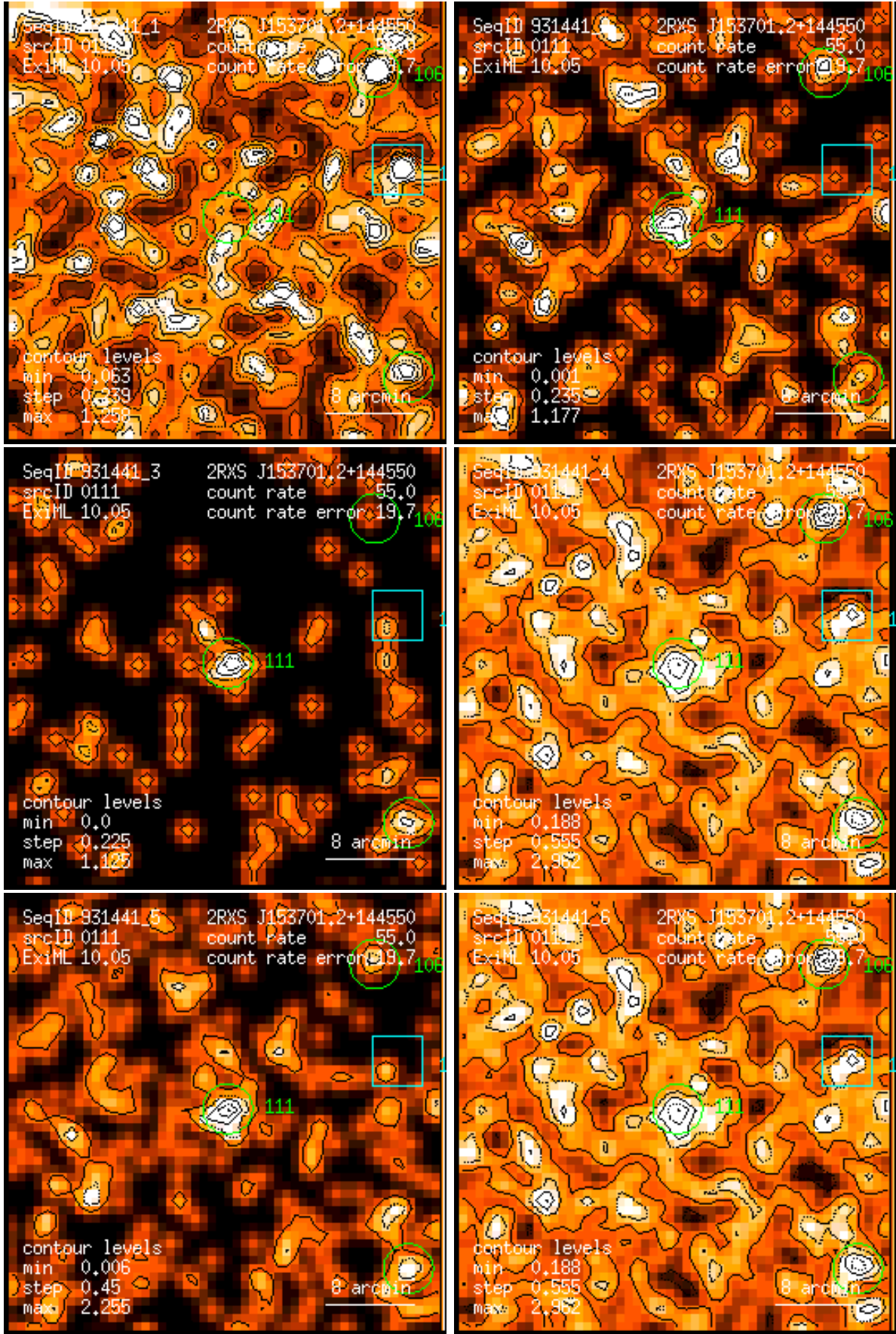
Figure 111: RASS 931441: detection 0111: band rate images, Gaussian filter: (1) PSPC channels 11 – 41, (2) 52 – 90, (3) 91 – 201, (4) 11 – 235, (5) 52 – 201, (6) 11 – 201. Broad band rates in counts/ks. Band rate contour levels in counts/ks/arcmin 2 .
