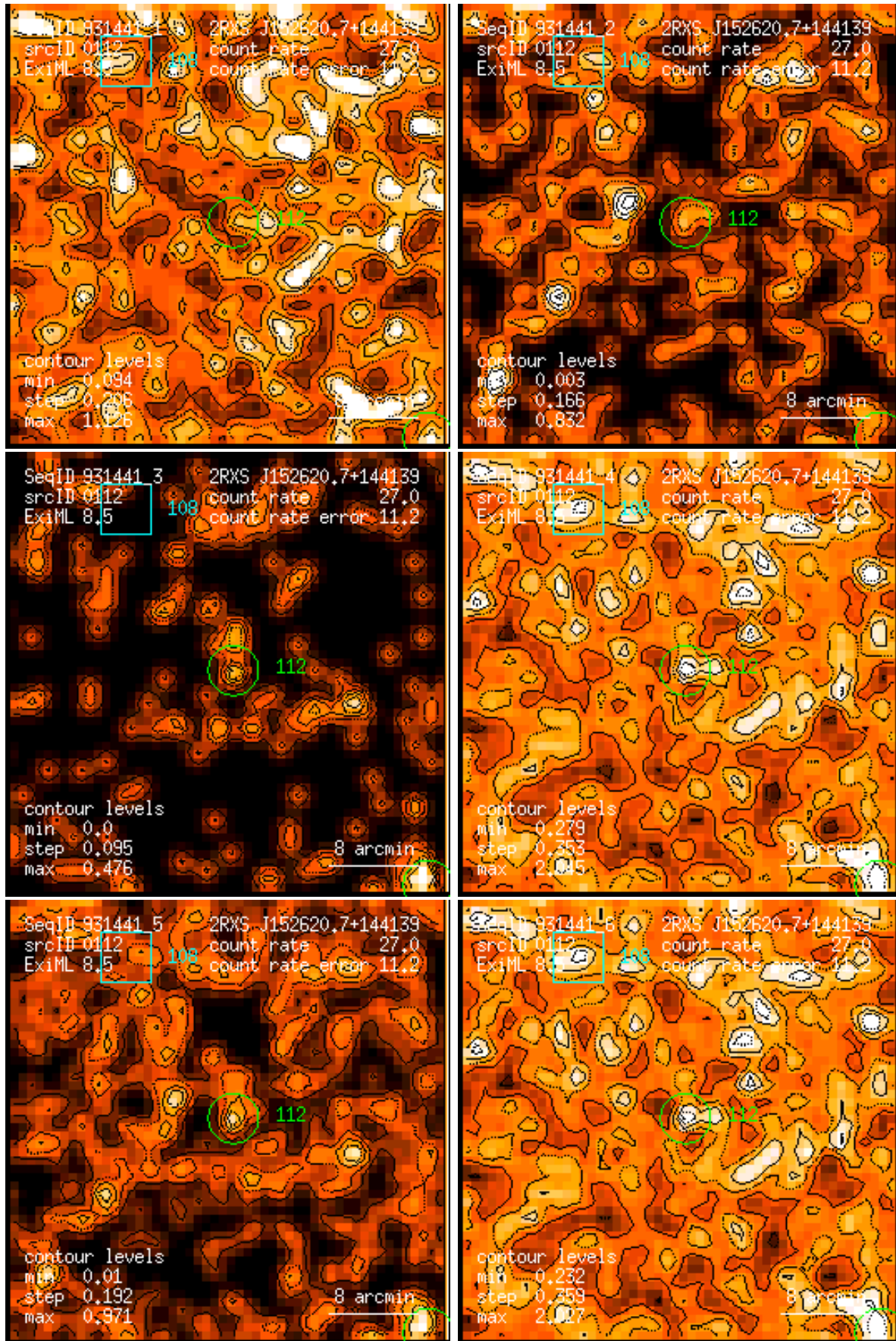
Figure 112: RASS 931441: detection 0112: band rate images, Gaussian filter: (1) PSPC channels 11 – 41, (2) 52 – 90, (3) 91 – 201, (4) 11 – 235, (5) 52 – 201, (6) 11 – 201. Broad band rates in counts/ks. Band rate contour levels in counts/ks/arcmin 2 .
