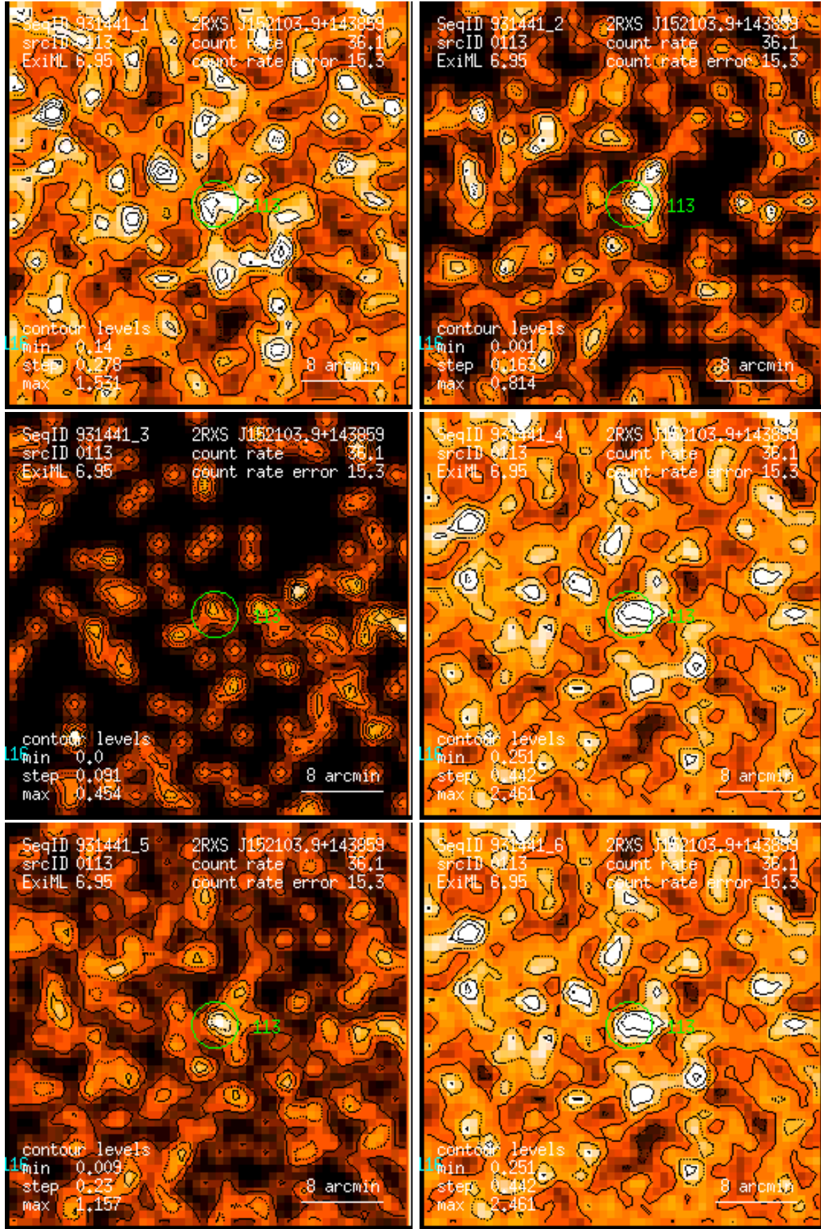
Figure 113: RASS 931441: detection 0113: band rate images, Gaussian filter: (1) PSPC channels 11 – 41, (2) 52 – 90, (3) 91 – 201, (4) 11 – 235, (5) 52 – 201, (6) 11 – 201. Broad band rates in counts/ks. Band rate contour levels in counts/ks/arcmin 2 .
