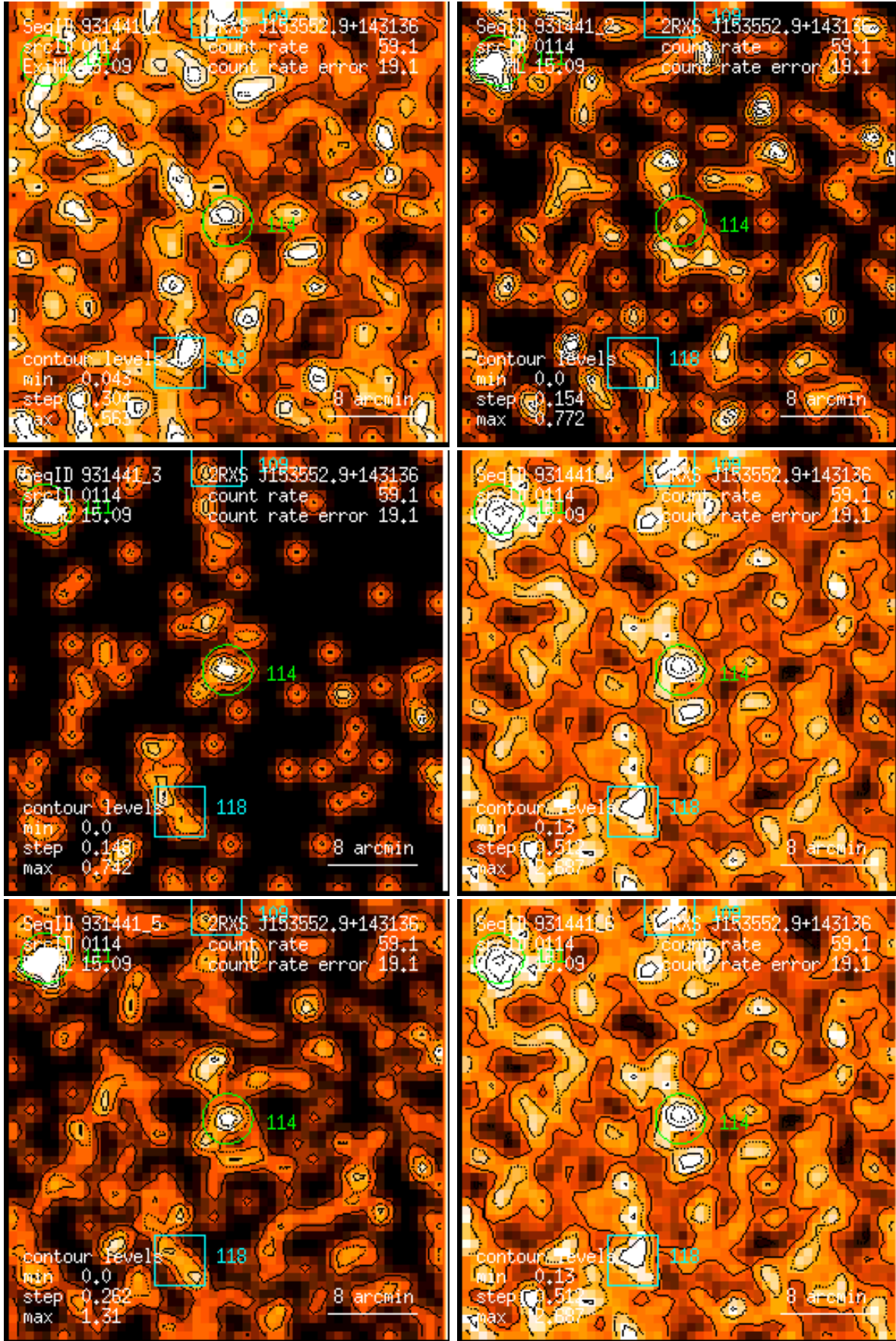
Figure 114: RASS 931441: detection 0114: band rate images, Gaussian filter: (1) PSPC channels 11 – 41, (2) 52 – 90, (3) 91 – 201, (4) 11 – 235, (5) 52 – 201, (6) 11 – 201. Broad band rates in counts/ks. Band rate contour levels in counts/ks/arcmin 2 .
