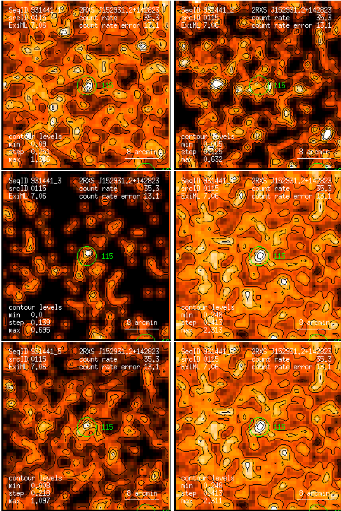
Figure 115: RASS 931441: detection 0115: band rate images, Gaussian filter: (1) PSPC channels 11 – 41, (2) 52 – 90, (3) 91 – 201, (4) 11 – 235, (5) 52 – 201, (6) 11 – 201. Broad band rates in counts/ks. Band rate contour levels in counts/ks/arcmin 2 .
