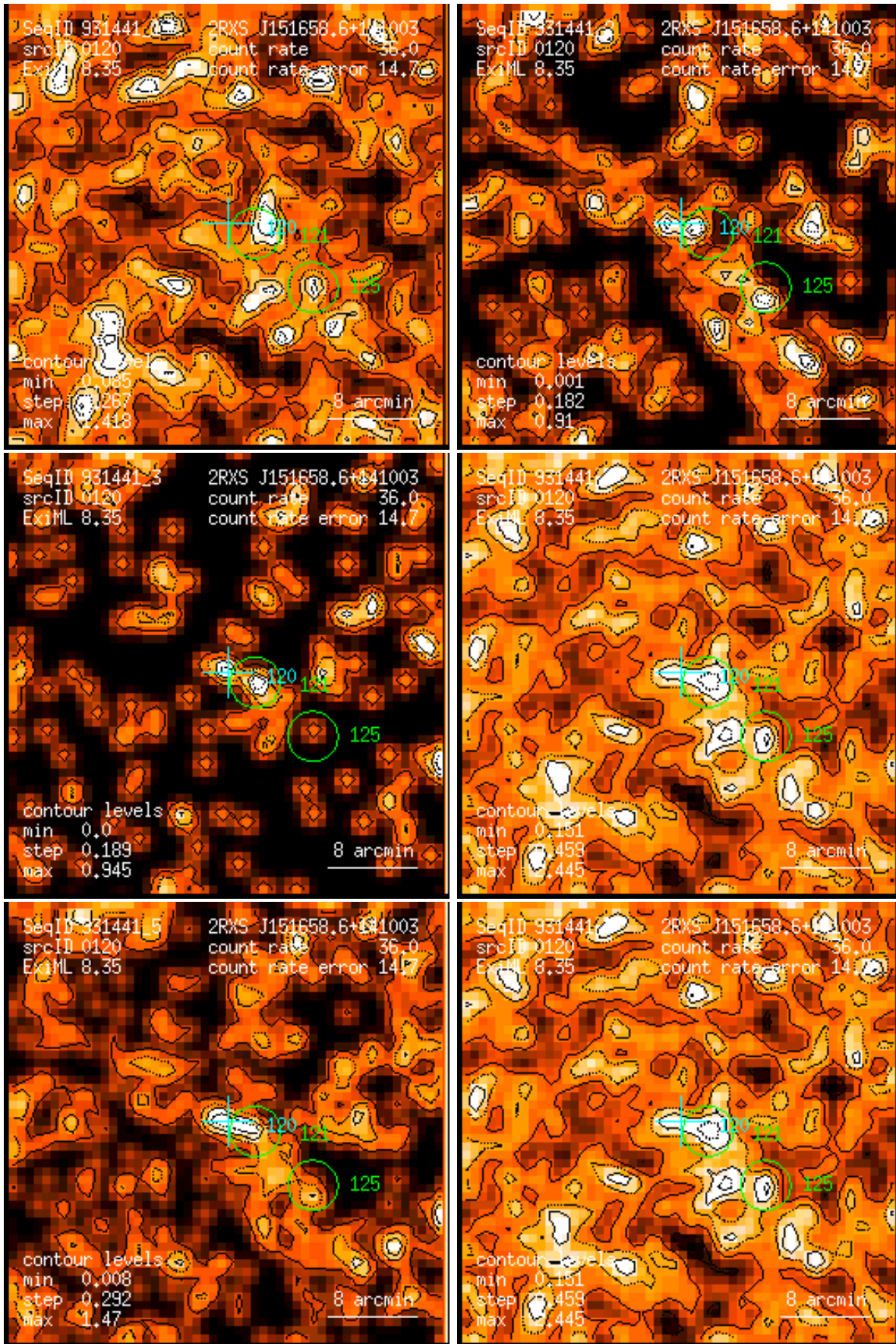
Figure 120: RASS 931441: detection 0120: band rate images, Gaussian filter: (1) PSPC channels 11 – 41, (2) 52 – 90, (3) 91 – 201, (4) 11 – 235, (5) 52 – 201, (6) 11 – 201. Broad band rates in counts/ks. Band rate contour levels in counts/ks/arcmin 2 .
