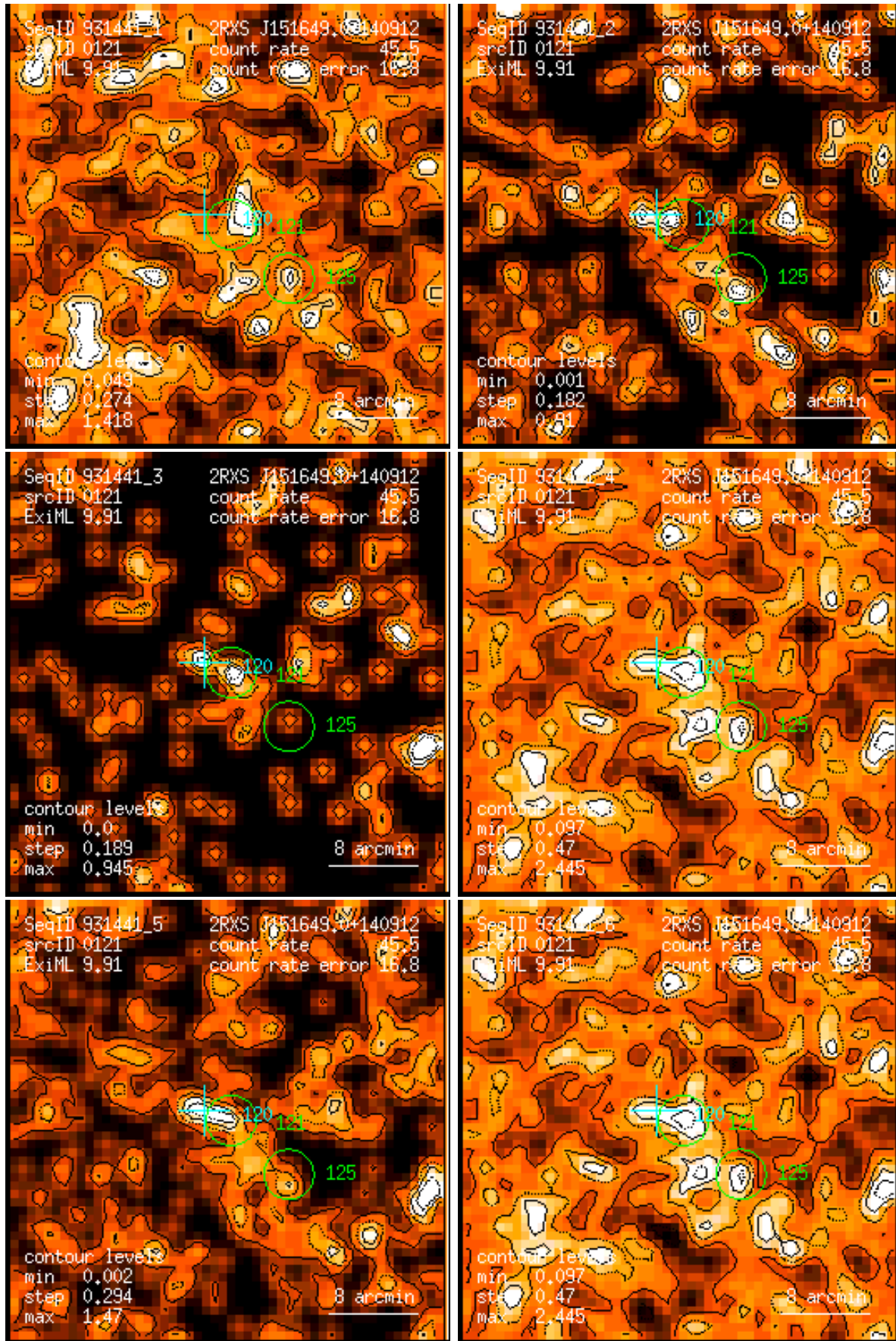
Figure 121: RASS 931441: detection 0121: band rate images, Gaussian filter: (1) PSPC channels 11 – 41, (2) 52 – 90, (3) 91 – 201, (4) 11 – 235, (5) 52 – 201, (6) 11 – 201. Broad band rates in counts/ks. Band rate contour levels in counts/ks/arcmin 2 .
