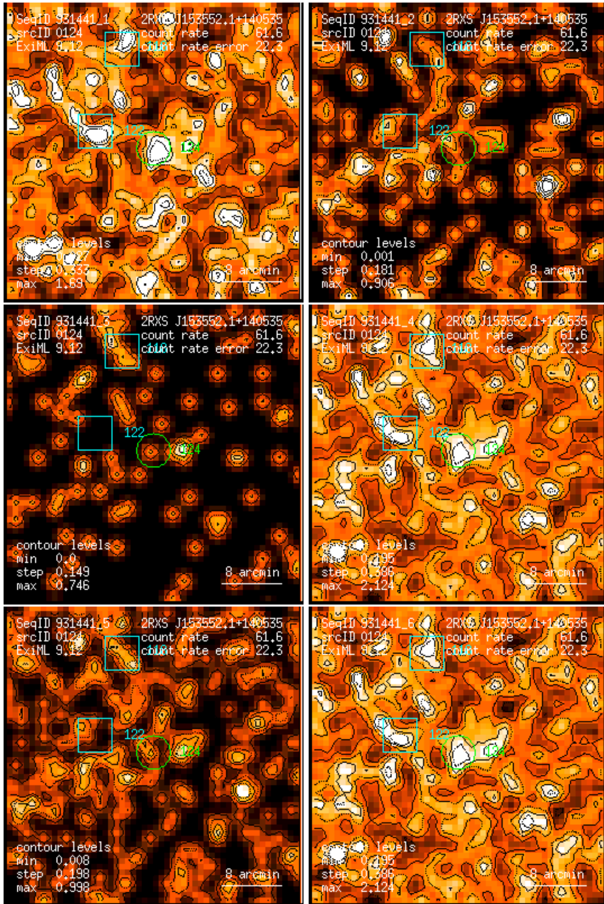
Figure 124: RASS 931441: detection 0124: band rate images, Gaussian filter: (1) PSPC channels 11 – 41, (2) 52 – 90, (3) 91 – 201, (4) 11 – 235, (5) 52 – 201, (6) 11 – 201. Broad band rates in counts/ks. Band rate contour levels in counts/ks/arcmin 2 .
