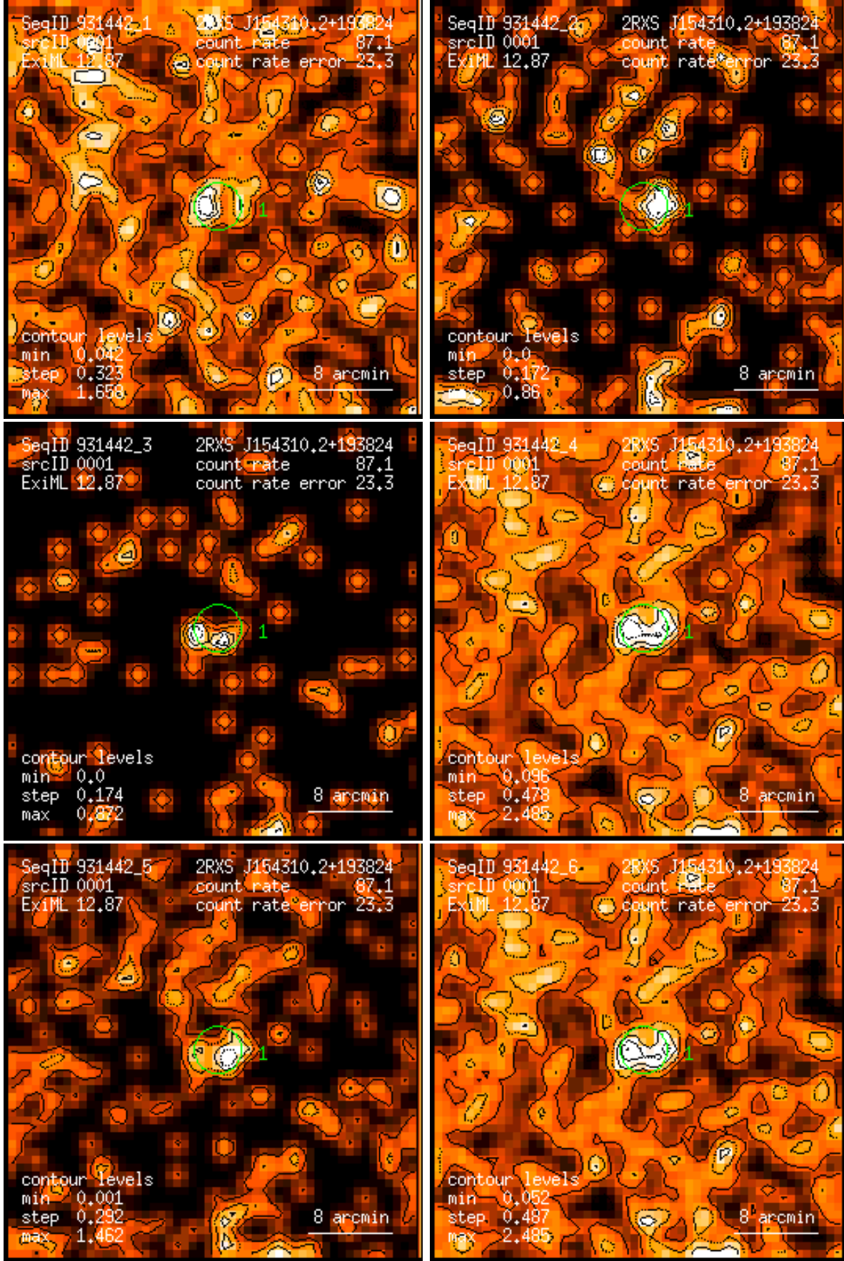
Figure 1: RASS 931442: detection 0001: band rate images, Gaussian filter: (1) PSPC channels 11 – 41, (2) 52 – 90, (3) 91 – 201, (4) 11 – 235, (5) 52 – 201, (6) 11 – 201. Broad band rates in counts/ks. Band rate contour levels in counts/ks/arcmin 2 .
