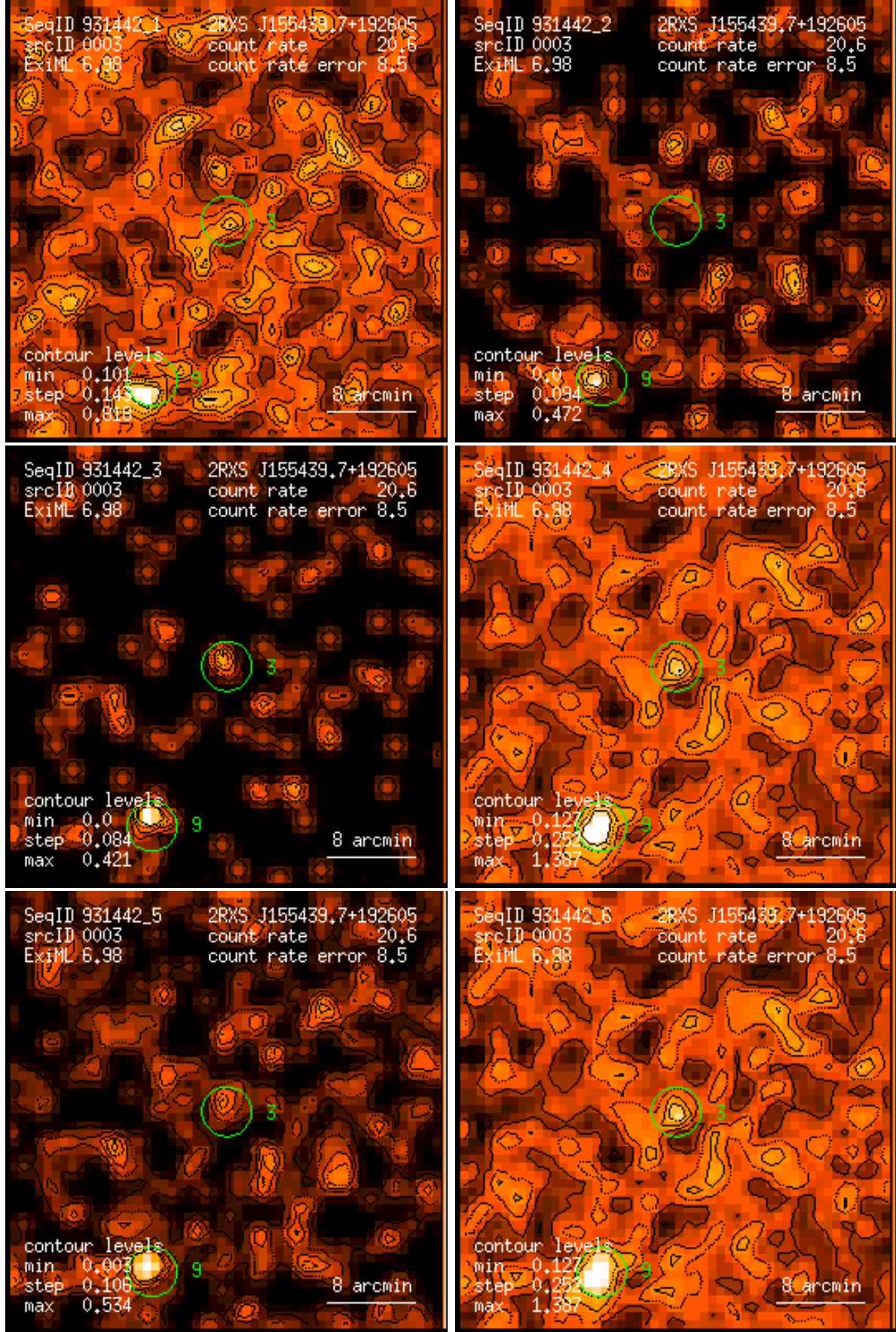
Figure 3: RASS 931442: detection 0003: band rate images, Gaussian filter: (1) PSPC channels 11 – 41, (2) 52 – 90, (3) 91 – 201, (4) 11 – 235, (5) 52 – 201, (6) 11 – 201. Broad band rates in counts/ks. Band rate contour levels in counts/ks/arcmin 2 .
