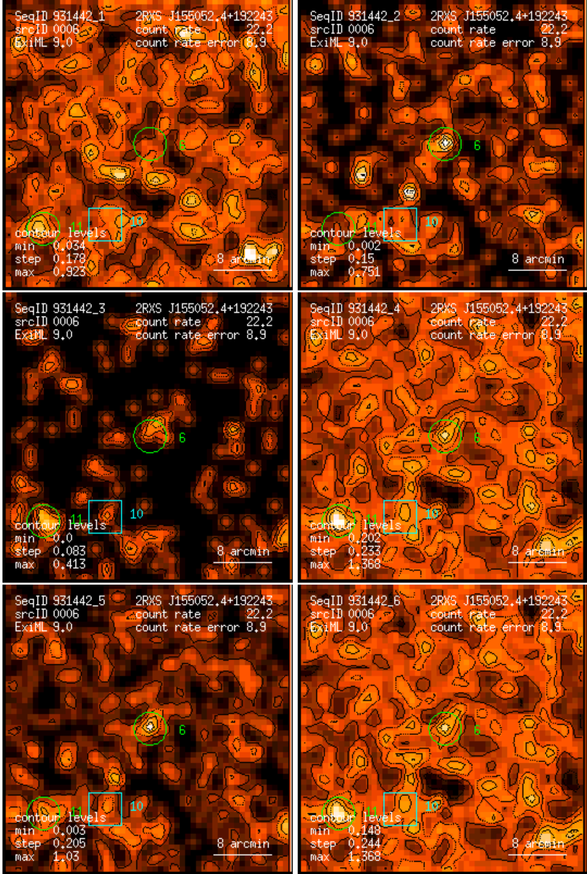
Figure 6: RASS 931442: detection 0006: band rate images, Gaussian filter: (1) PSPC channels 11 – 41, (2) 52 – 90, (3) 91 – 201, (4) 11 – 235, (5) 52 – 201, (6) 11 – 201. Broad band rates in counts/ks. Band rate contour levels in counts/ks/arcmin 2 .
