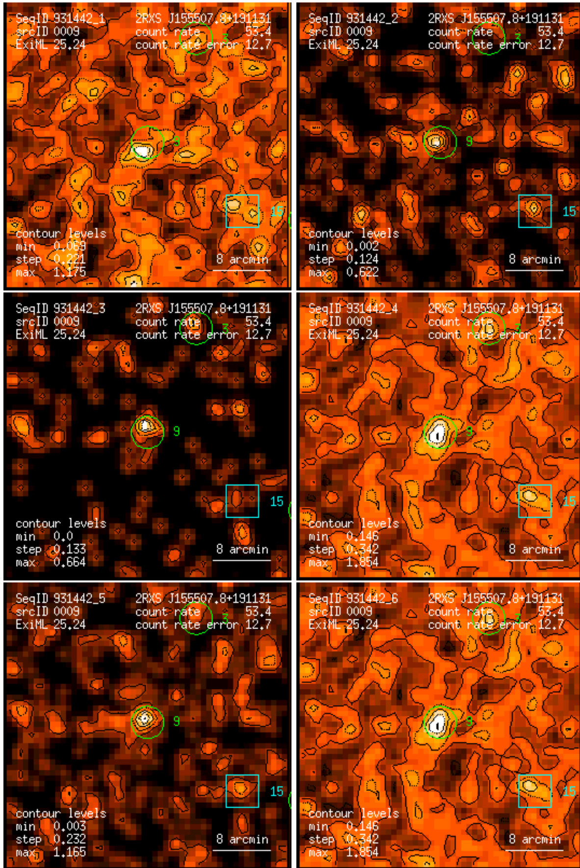
Figure 9: RASS 931442: detection 0009: band rate images, Gaussian filter: (1) PSPC channels 11 – 41, (2) 52 – 90, (3) 91 – 201, (4) 11 – 235, (5) 52 – 201, (6) 11 – 201. Broad band rates in counts/ks. Band rate contour levels in counts/ks/arcmin 2 .
