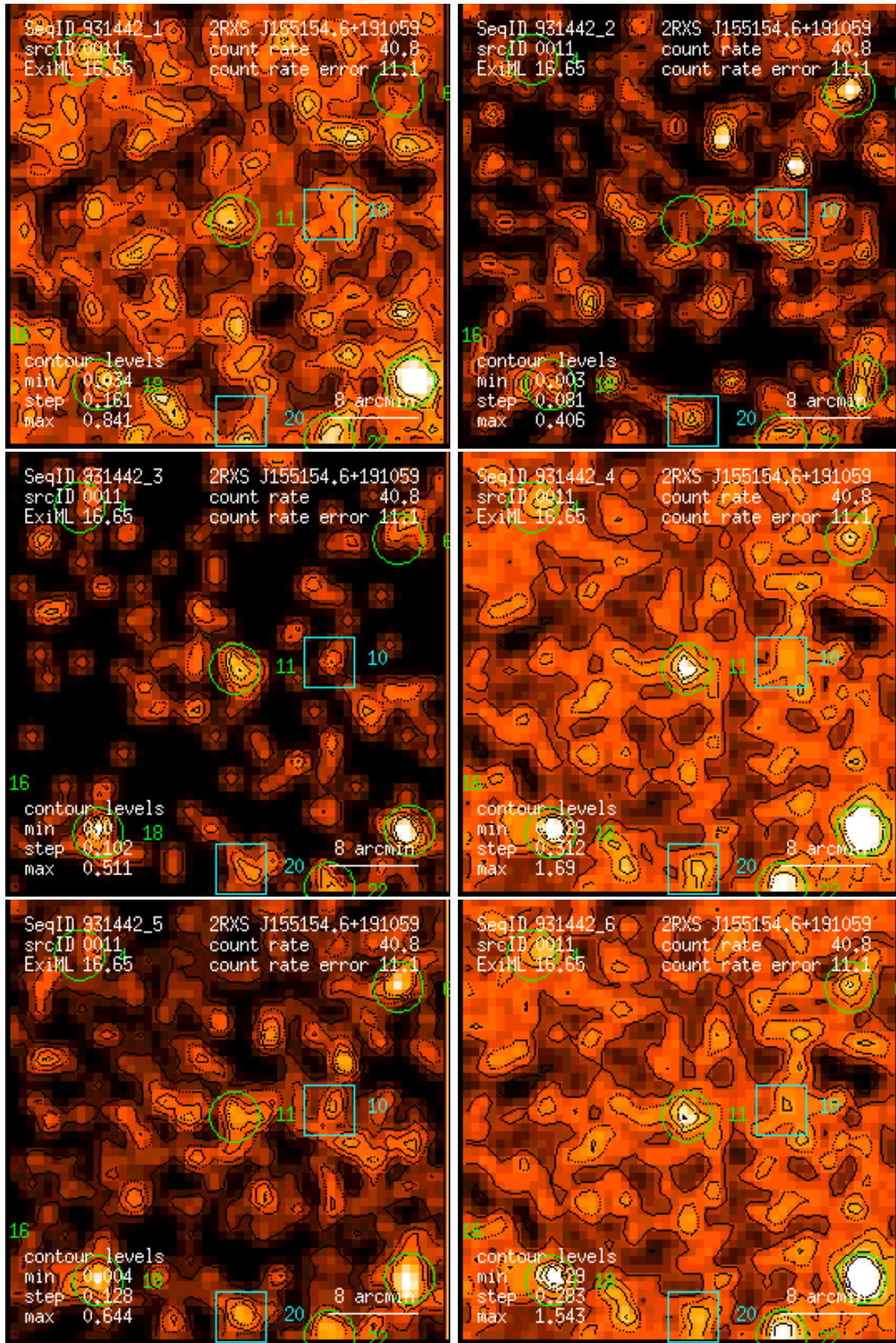
Figure 11: RASS 931442: detection 0011: band rate images, Gaussian filter: (1) PSPC channels 11 – 41, (2) 52 – 90, (3) 91 – 201, (4) 11 – 235, (5) 52 – 201, (6) 11 – 201. Broad band rates in counts/ks. Band rate contour levels in counts/ks/arcmin 2 .
