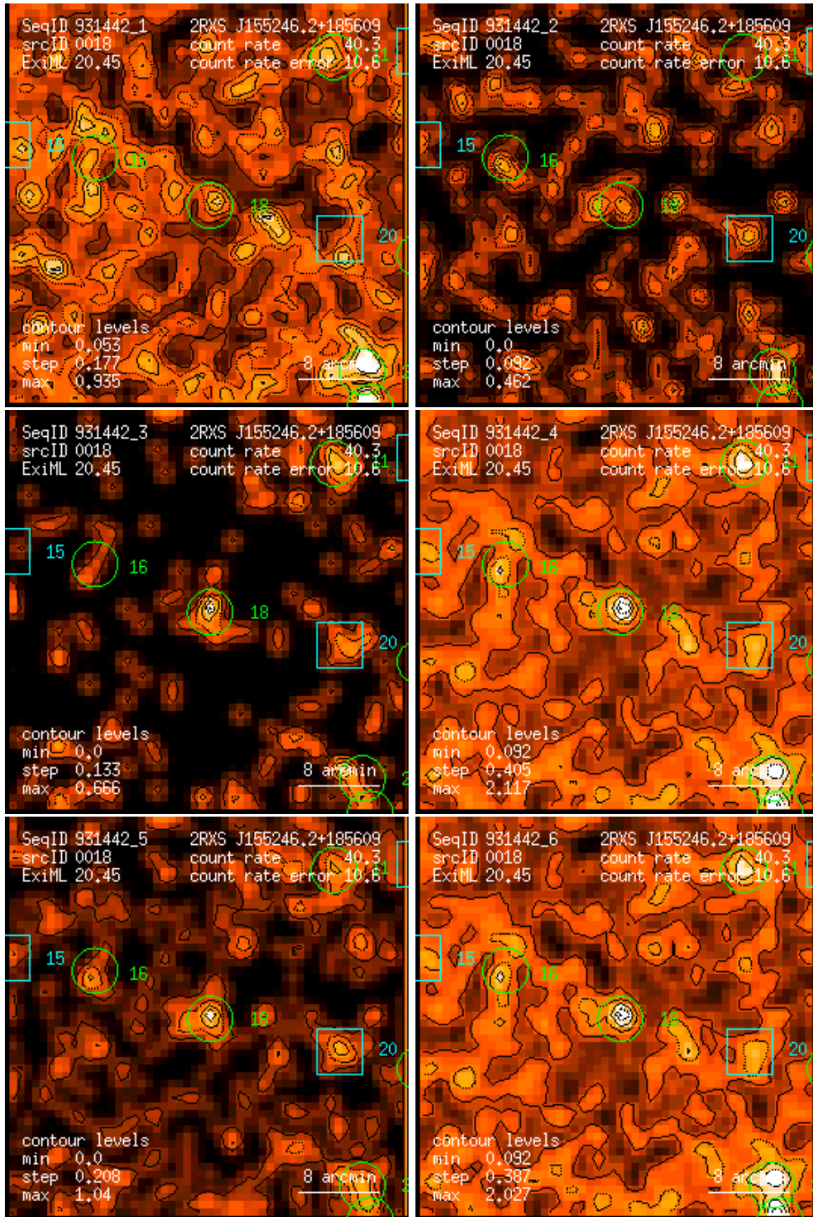
Figure 18: RASS 931442: detection 0018: band rate images, Gaussian filter: (1) PSPC channels 11 – 41, (2) 52 – 90, (3) 91 – 201, (4) 11 – 235, (5) 52 – 201, (6) 11 – 201. Broad band rates in counts/ks. Band rate contour levels in counts/ks/arcmin 2 .
