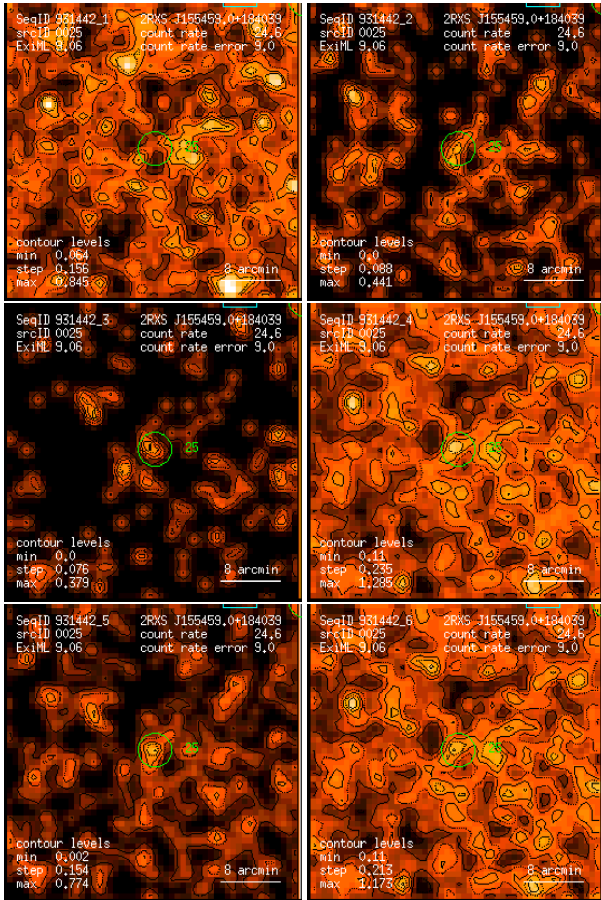
Figure 25: RASS 931442: detection 0025: band rate images, Gaussian filter: (1) PSPC channels 11 – 41, (2) 52 – 90, (3) 91 – 201, (4) 11 – 235, (5) 52 – 201, (6) 11 – 201. Broad band rates in counts/ks. Band rate contour levels in counts/ks/arcmin 2 .
