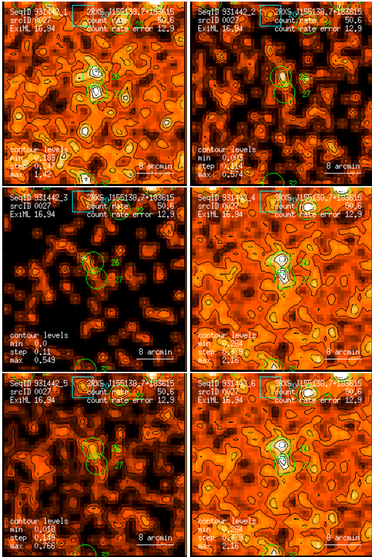
Figure 27: RASS 931442: detection 0027: band rate images, Gaussian filter: (1) PSPC channels 11 – 41, (2) 52 – 90, (3) 91 – 201, (4) 11 – 235, (5) 52 – 201, (6) 11 – 201. Broad band rates in counts/ks. Band rate contour levels in counts/ks/arcmin 2 .
