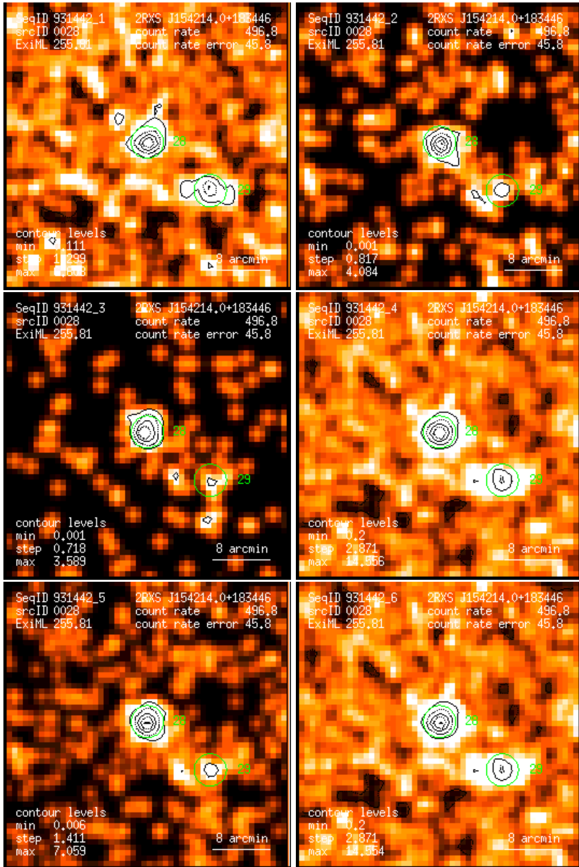
Figure 28: RASS 931442: detection 0028: band rate images, Gaussian filter: (1) PSPC channels 11 – 41, (2) 52 – 90, (3) 91 – 201, (4) 11 – 235, (5) 52 – 201, (6) 11 – 201. Broad band rates in counts/ks. Band rate contour levels in counts/ks/arcmin 2 .
