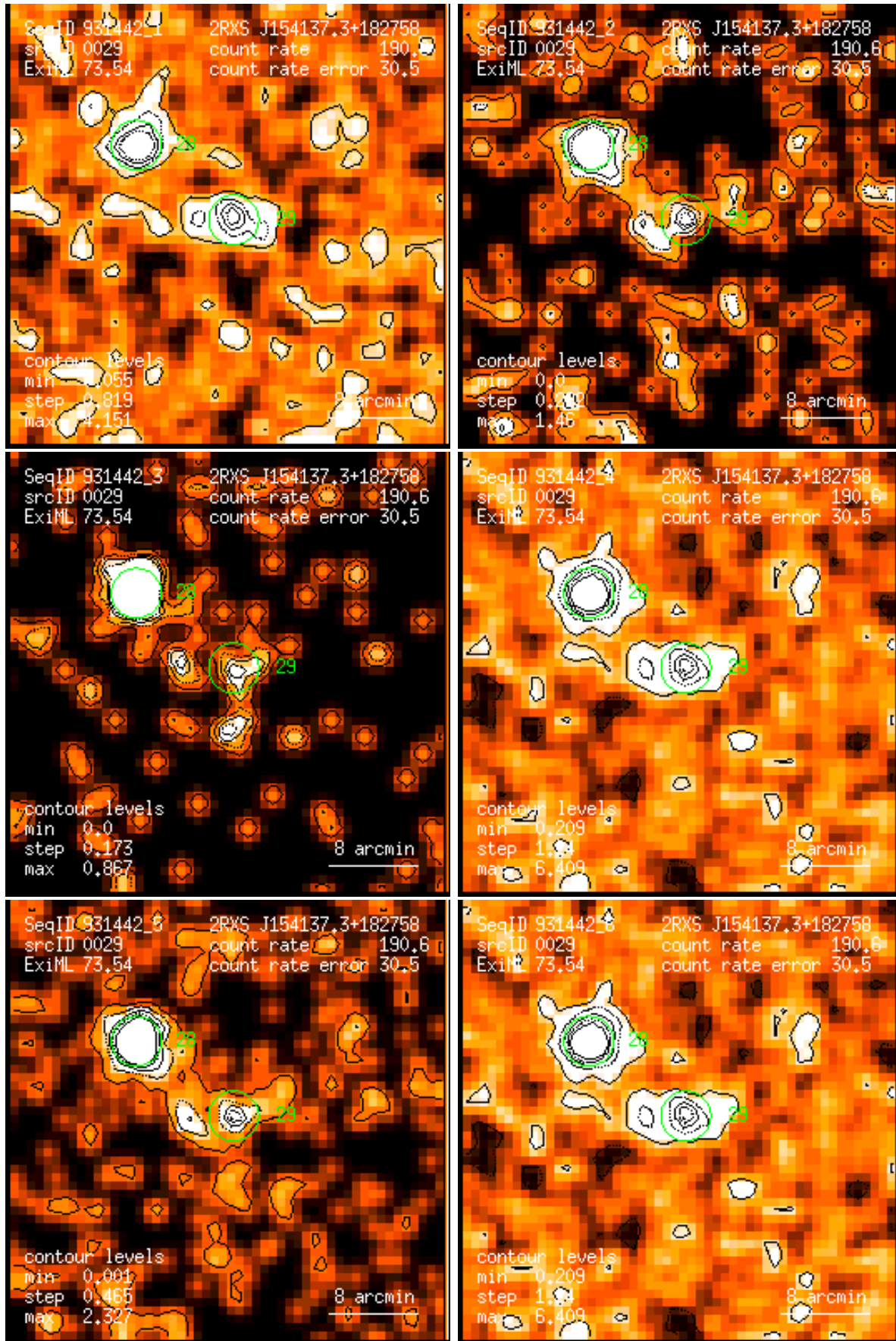
Figure 29: RASS 931442: detection 0029: band rate images, Gaussian filter: (1) PSPC channels 11 – 41, (2) 52 – 90, (3) 91 – 201, (4) 11 – 235, (5) 52 – 201, (6) 11 – 201. Broad band rates in counts/ks. Band rate contour levels in counts/ks/arcmin 2 .
