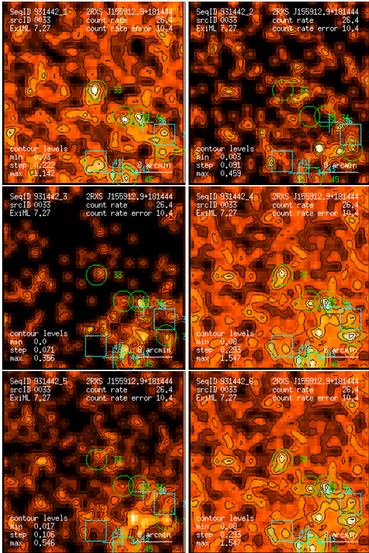
Figure 33: RASS 931442: detection 0033: band rate images, Gaussian filter: (1) PSPC channels 11 – 41, (2) 52 – 90, (3) 91 – 201, (4) 11 – 235, (5) 52 – 201, (6) 11 – 201. Broad band rates in counts/ks. Band rate contour levels in counts/ks/arcmin 2 .
