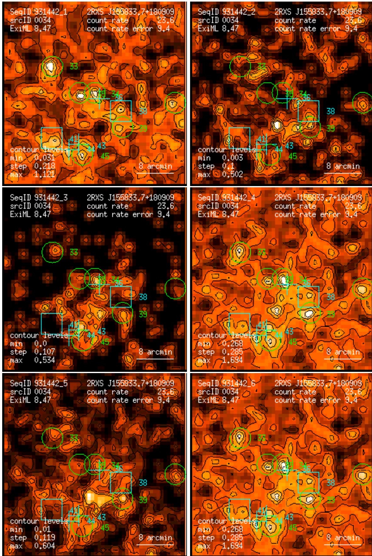
Figure 34: RASS 931442: detection 0034: band rate images, Gaussian filter: (1) PSPC channels 11 – 41, (2) 52 – 90, (3) 91 – 201, (4) 11 – 235, (5) 52 – 201, (6) 11 – 201. Broad band rates in counts/ks. Band rate contour levels in counts/ks/arcmin 2 .
