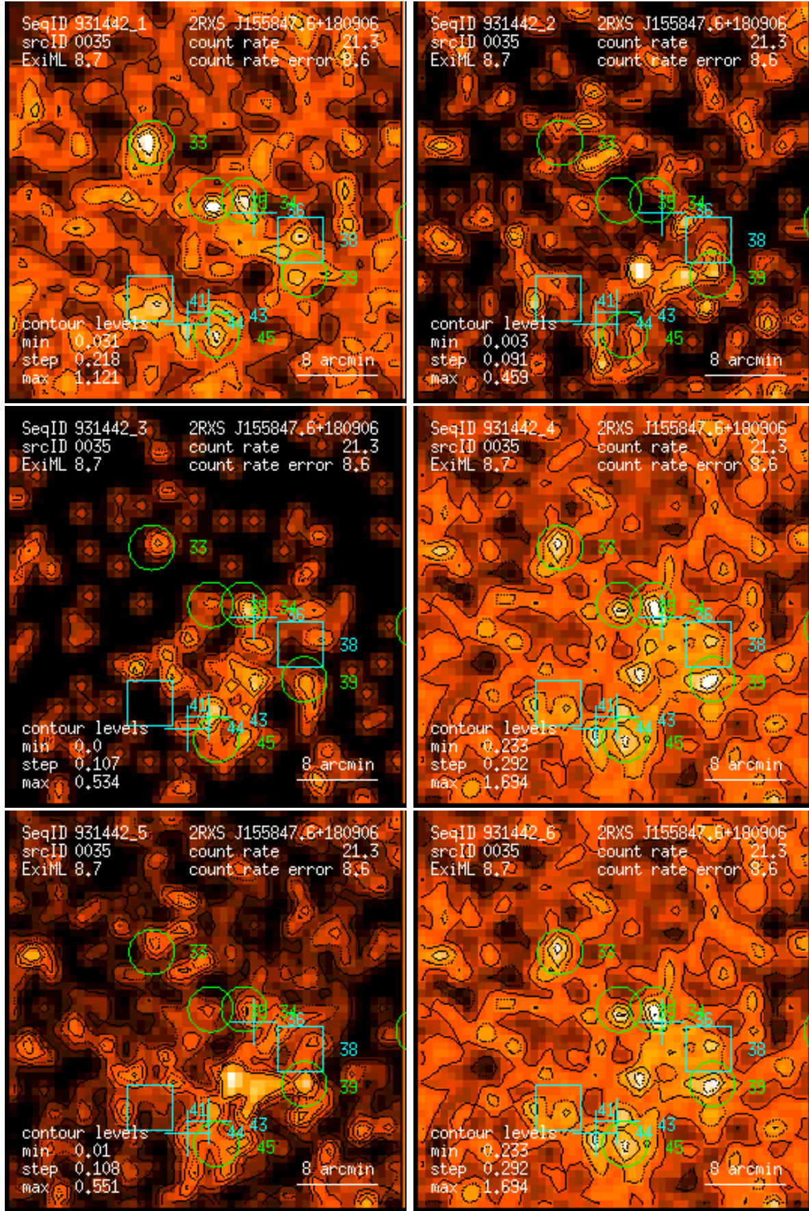
Figure 35: RASS 931442: detection 0035: band rate images, Gaussian filter: (1) PSPC channels 11 – 41, (2) 52 – 90, (3) 91 – 201, (4) 11 – 235, (5) 52 – 201, (6) 11 – 201. Broad band rates in counts/ks. Band rate contour levels in counts/ks/arcmin 2 .
