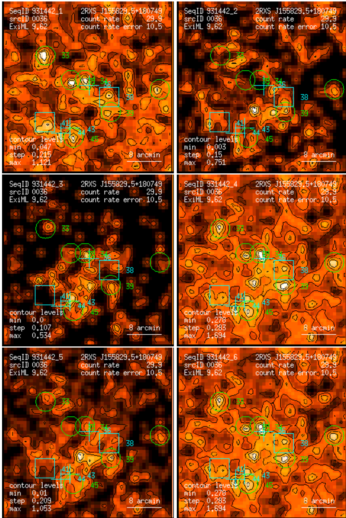
Figure 36: RASS 931442: detection 0036: band rate images, Gaussian filter: (1) PSPC channels 11 – 41, (2) 52 – 90, (3) 91 – 201, (4) 11 – 235, (5) 52 – 201, (6) 11 – 201. Broad band rates in counts/ks. Band rate contour levels in counts/ks/arcmin 2 .
