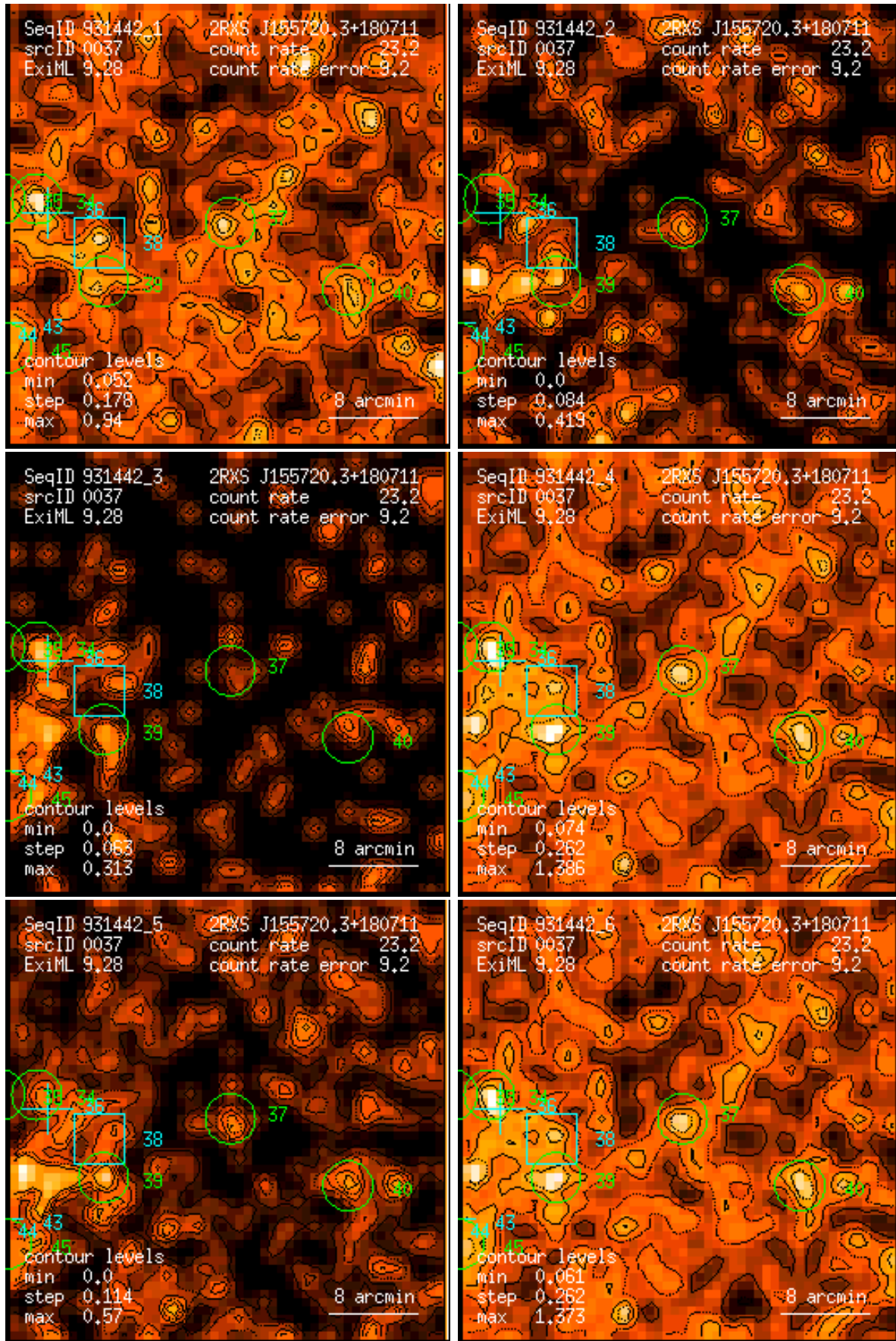
Figure 37: RASS 931442: detection 0037: band rate images, Gaussian filter: (1) PSPC channels 11 – 41, (2) 52 – 90, (3) 91 – 201, (4) 11 – 235, (5) 52 – 201, (6) 11 – 201. Broad band rates in counts/ks. Band rate contour levels in counts/ks/arcmin 2 .
