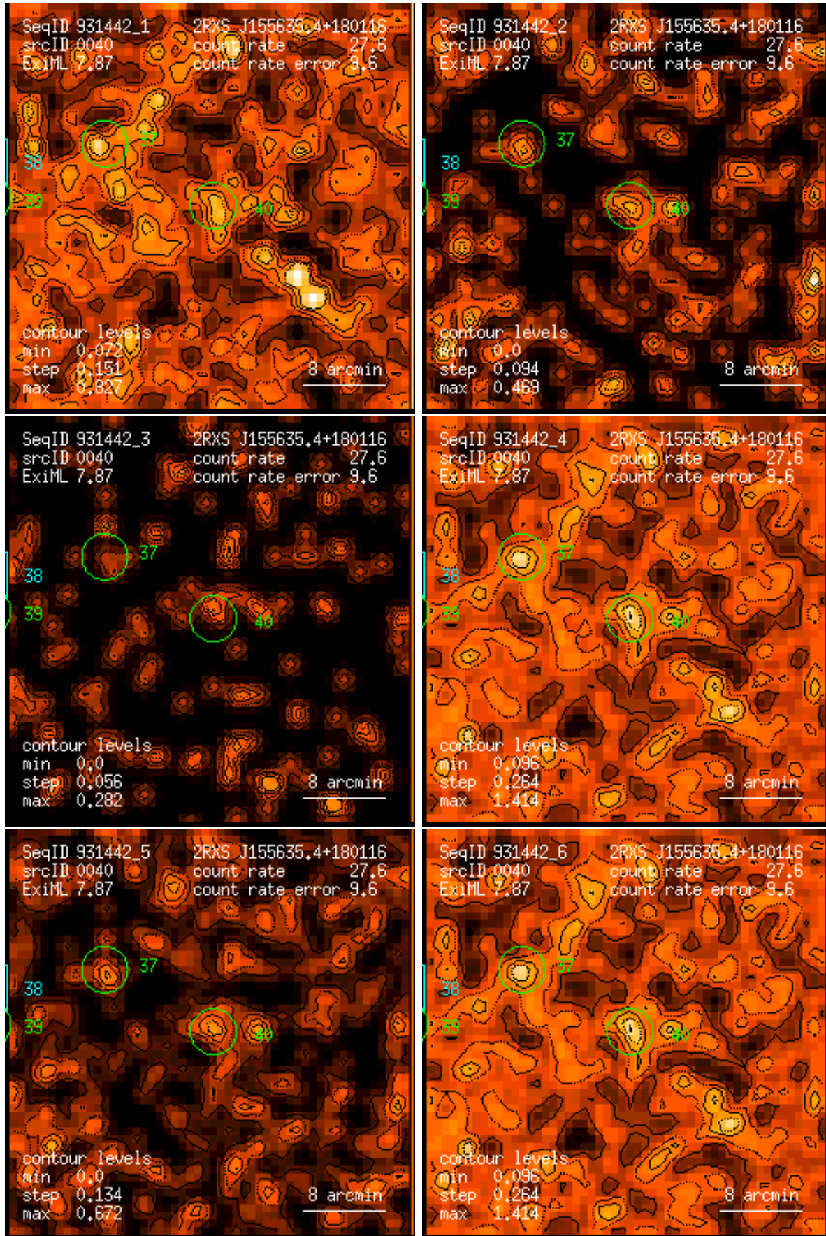
Figure 40: RASS 931442: detection 0040: band rate images, Gaussian filter: (1) PSPC channels 11 – 41, (2) 52 – 90, (3) 91 – 201, (4) 11 – 235, (5) 52 – 201, (6) 11 – 201. Broad band rates in counts/ks. Band rate contour levels in counts/ks/arcmin 2 .
