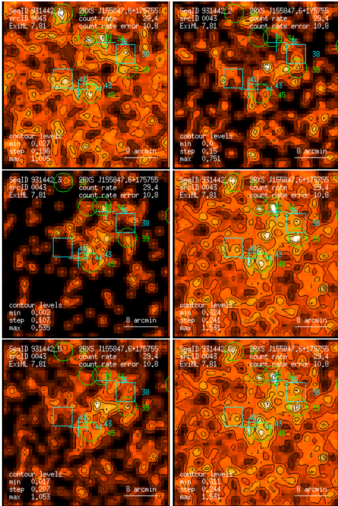
Figure 43: RASS 931442: detection 0043: band rate images, Gaussian filter: (1) PSPC channels 11 – 41, (2) 52 – 90, (3) 91 – 201, (4) 11 – 235, (5) 52 – 201, (6) 11 – 201. Broad band rates in counts/ks. Band rate contour levels in counts/ks/arcmin 2 .
