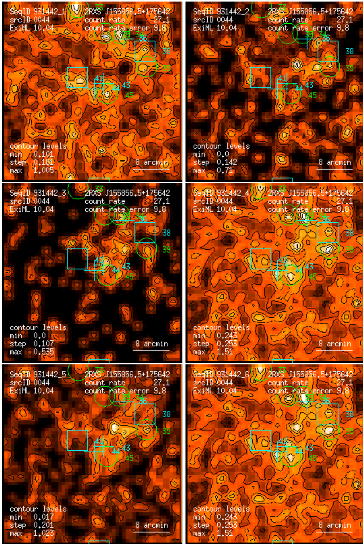
Figure 44: RASS 931442: detection 0044: band rate images, Gaussian filter: (1) PSPC channels 11 – 41, (2) 52 – 90, (3) 91 – 201, (4) 11 – 235, (5) 52 – 201, (6) 11 – 201. Broad band rates in counts/ks. Band rate contour levels in counts/ks/arcmin 2 .
