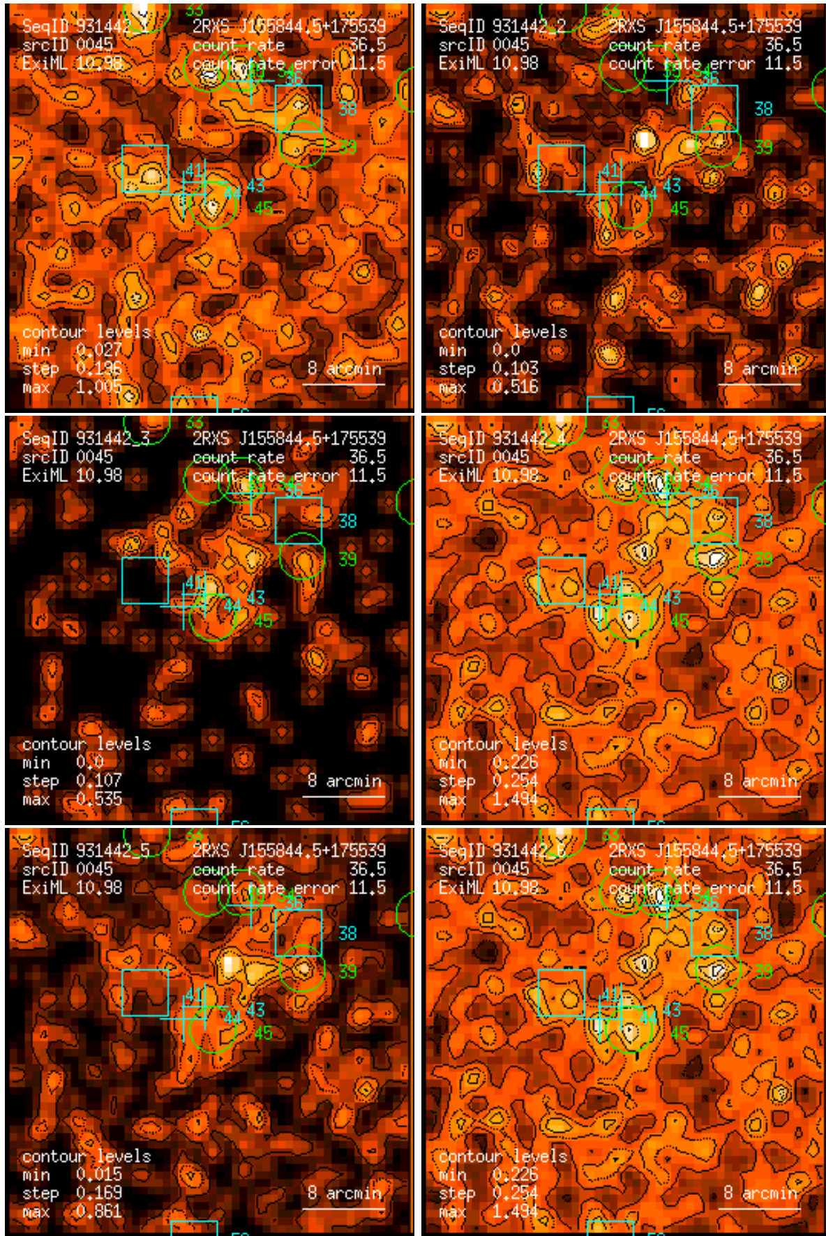
Figure 45: RASS 931442: detection 0045: band rate images, Gaussian filter: (1) PSPC channels 11 – 41, (2) 52 – 90, (3) 91 – 201, (4) 11 – 235, (5) 52 – 201, (6) 11 – 201. Broad band rates in counts/ks. Band rate contour levels in counts/ks/arcmin 2 .
