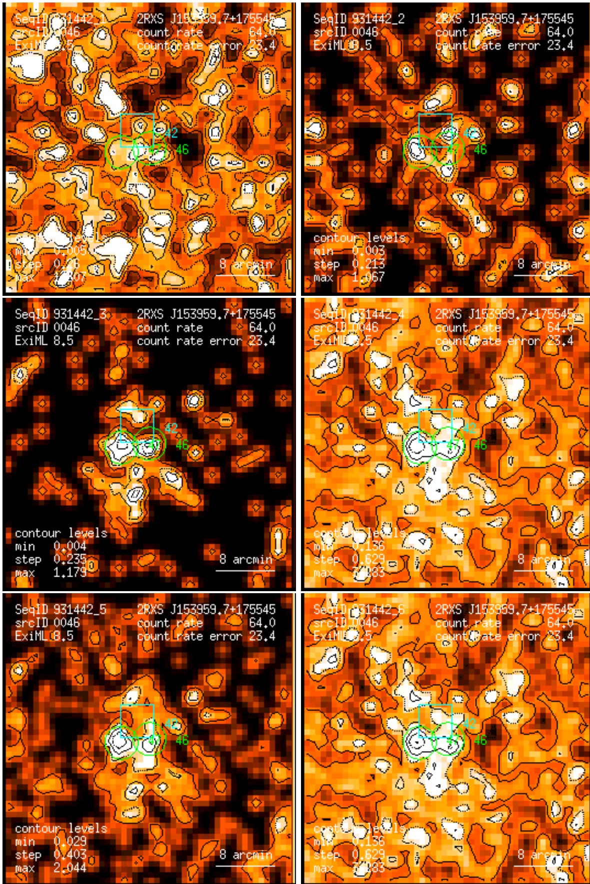
Figure 46: RASS 931442: detection 0046: band rate images, Gaussian filter: (1) PSPC channels 11 – 41, (2) 52 – 90, (3) 91 – 201, (4) 11 – 235, (5) 52 – 201, (6) 11 – 201. Broad band rates in counts/ks. Band rate contour levels in counts/ks/arcmin 2 .
