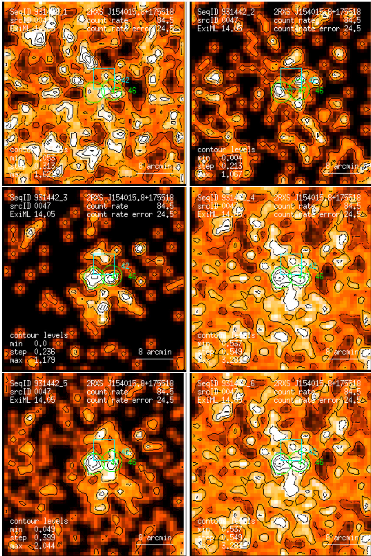
Figure 47: RASS 931442: detection 0047: band rate images, Gaussian filter: (1) PSPC channels 11 – 41, (2) 52 – 90, (3) 91 – 201, (4) 11 – 235, (5) 52 – 201, (6) 11 – 201. Broad band rates in counts/ks. Band rate contour levels in counts/ks/arcmin 2 .
