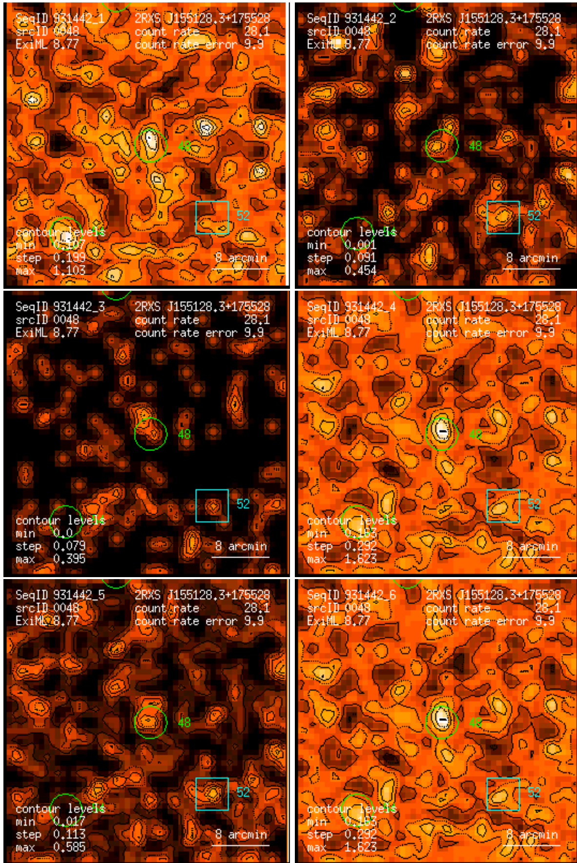
Figure 48: RASS 931442: detection 0048: band rate images, Gaussian filter: (1) PSPC channels 11 – 41, (2) 52 – 90, (3) 91 – 201, (4) 11 – 235, (5) 52 – 201, (6) 11 – 201. Broad band rates in counts/ks. Band rate contour levels in counts/ks/arcmin 2 .
