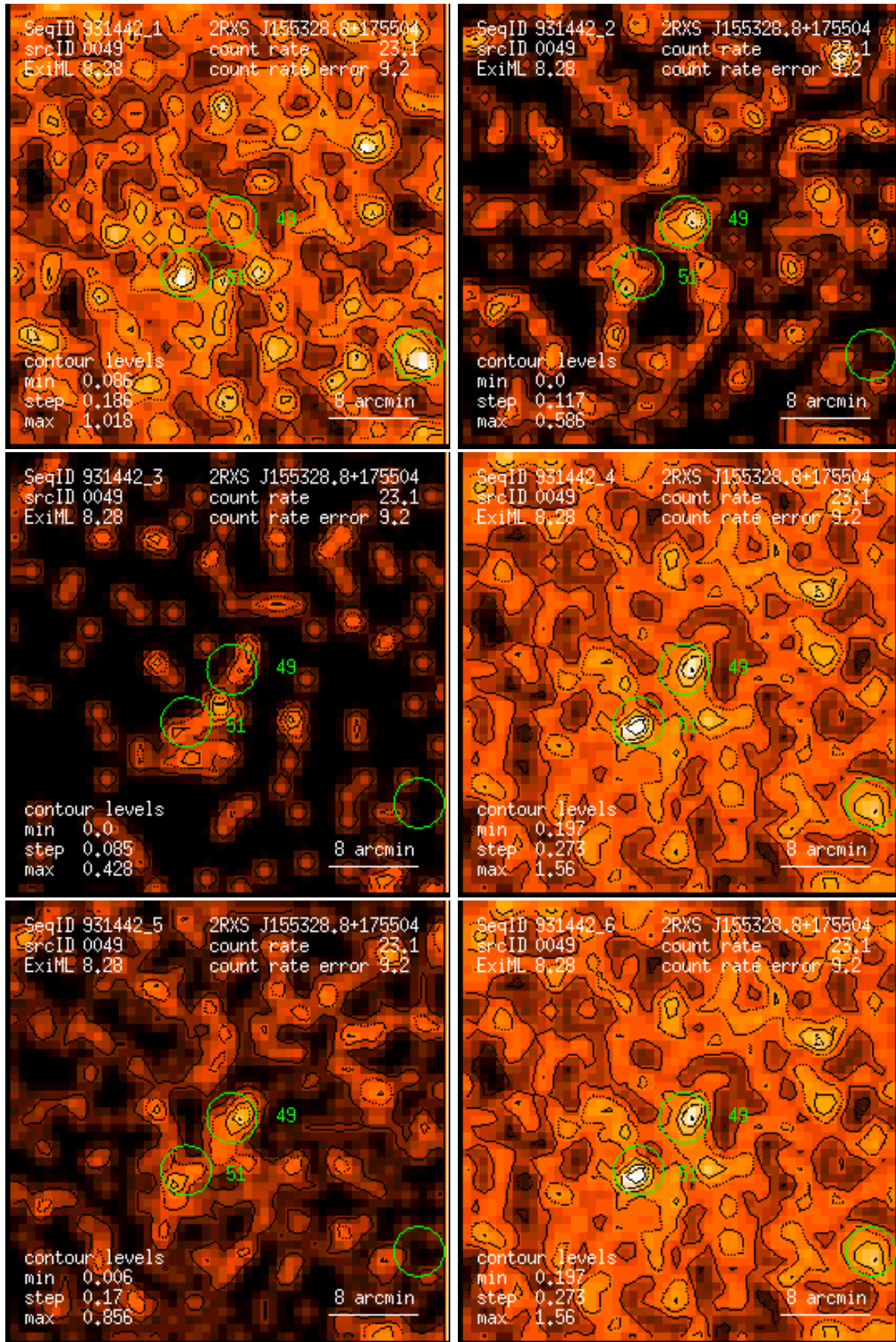
Figure 49: RASS 931442: detection 0049: band rate images, Gaussian filter: (1) PSPC channels 11 – 41, (2) 52 – 90, (3) 91 – 201, (4) 11 – 235, (5) 52 – 201, (6) 11 – 201. Broad band rates in counts/ks. Band rate contour levels in counts/ks/arcmin 2 .
