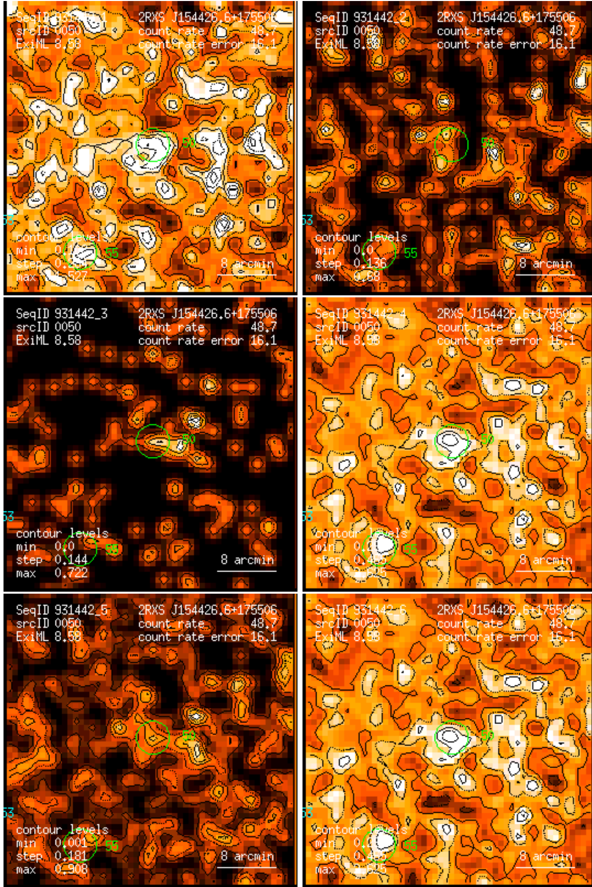
Figure 50: RASS 931442: detection 0050: band rate images, Gaussian filter: (1) PSPC channels 11 – 41, (2) 52 – 90, (3) 91 – 201, (4) 11 – 235, (5) 52 – 201, (6) 11 – 201. Broad band rates in counts/ks. Band rate contour levels in counts/ks/arcmin 2 .
