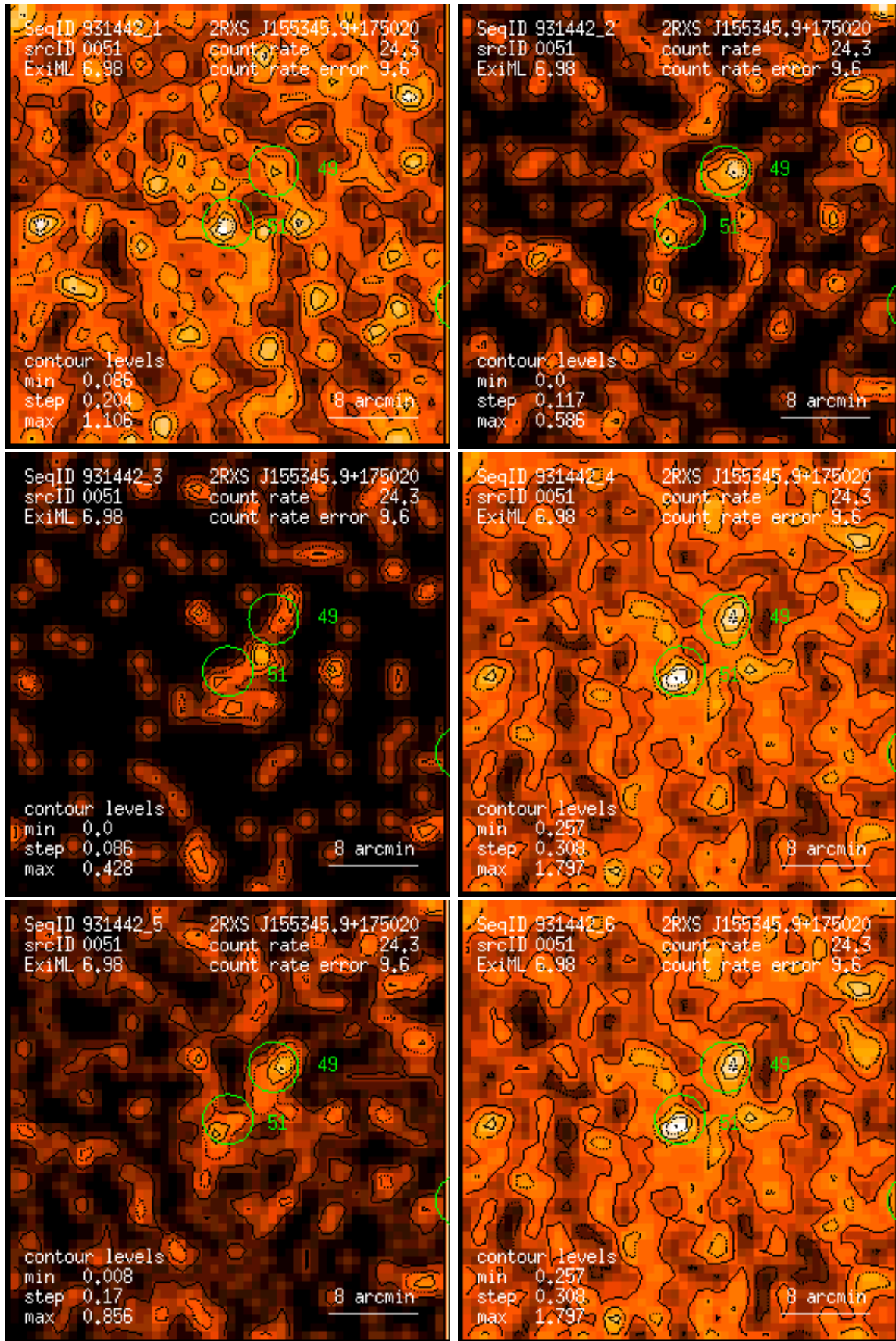
Figure 51: RASS 931442: detection 0051: band rate images, Gaussian filter: (1) PSPC channels 11 – 41, (2) 52 – 90, (3) 91 – 201, (4) 11 – 235, (5) 52 – 201, (6) 11 – 201. Broad band rates in counts/ks. Band rate contour levels in counts/ks/arcmin 2 .
