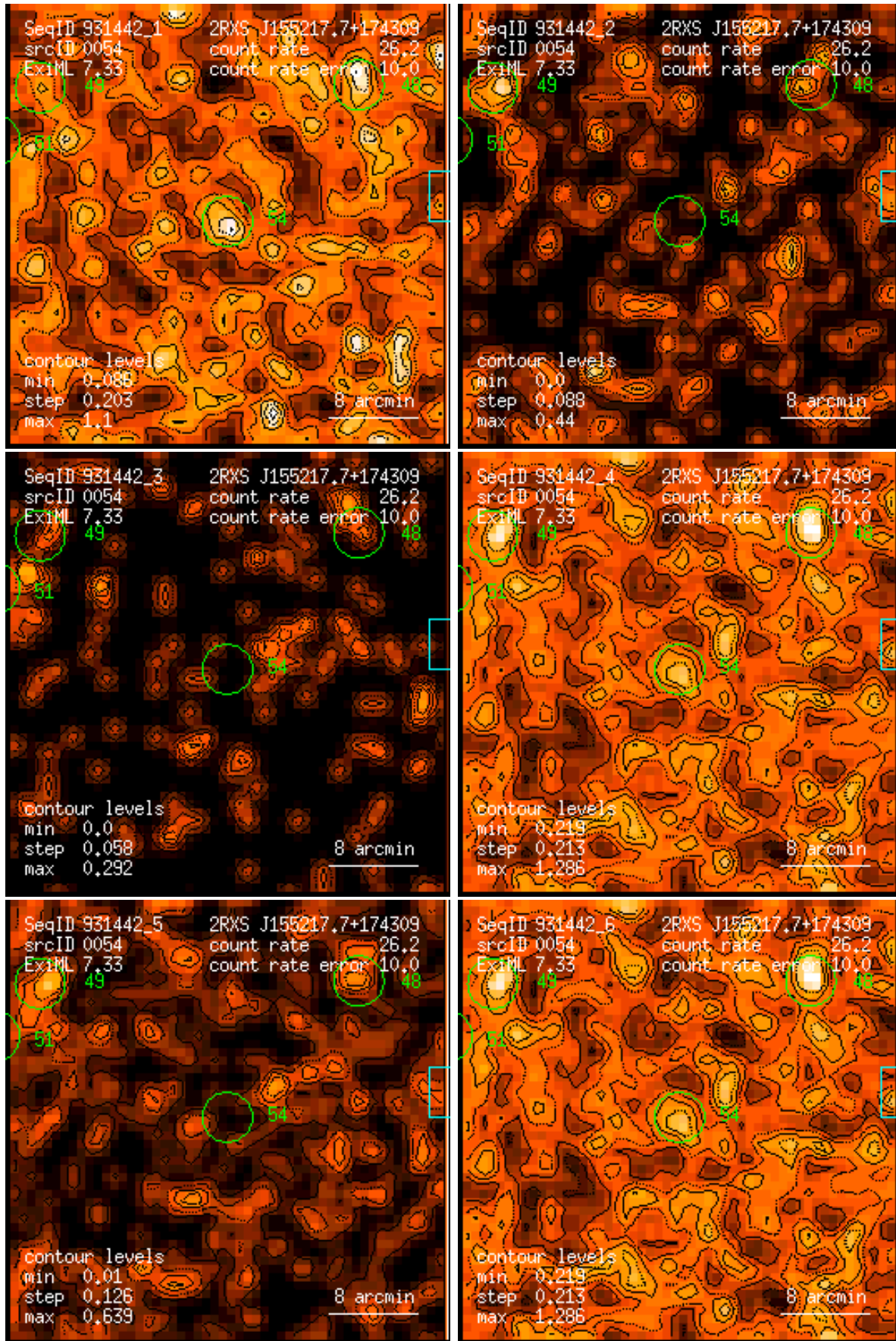
Figure 54: RASS 931442: detection 0054: band rate images, Gaussian filter: (1) PSPC channels 11 – 41, (2) 52 – 90, (3) 91 – 201, (4) 11 – 235, (5) 52 – 201, (6) 11 – 201. Broad band rates in counts/ks. Band rate contour levels in counts/ks/arcmin 2 .
